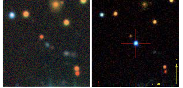
Fig. 1. Left: pre-SN image retrieved from the Dark Energy Camera Legacy Surveys (DR9). Right: image of SN 2020qlb taken on August 9, 2020 (61 rest frame days before peak) with the Liverpool Telescope in ugriz frames and stacked (Lupton et al. 2004) around the SN location. Each image is 45 by 45 arcsec.
