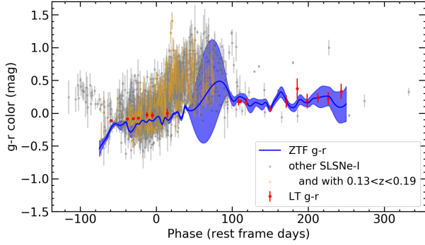
Fig. 7. SN 2020qlb g - r color evolution created from the ZTF- g and -r filter GP interpolations in Sect. 3.2 in blue and the g - r measurements with the LT in red. The gray background is a scatter plot of the 75 SLSNe-I and orange is for the 9 with 0.13 < z < 0.19 from Chen et al. (2022b, Fig. 13).
