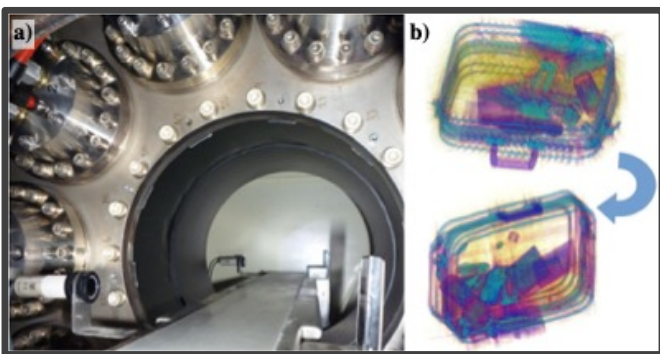
Fig. 3: a) Prototype baggage scanner that uses multiple X-ray sources and detectors (from [5]), allowing b) reconstruction of 3D images in real time (from [4]), meaning we can now leave liquids and laptops in bags at airport security.
