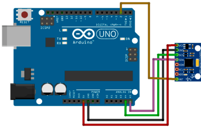
Fig. 4. Wiring diagram to Arduino UNO with MPU 6050.
