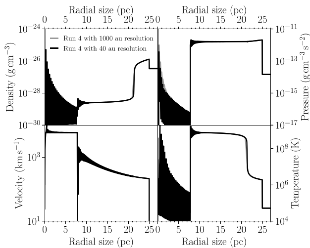
Figure 2. Comparing the dynamics of Run 4 (resolution of 1000 \text{ au cell}^{-1} ) and Run 4 with a resolution of 40 \text{ au cell}^{-1} .
