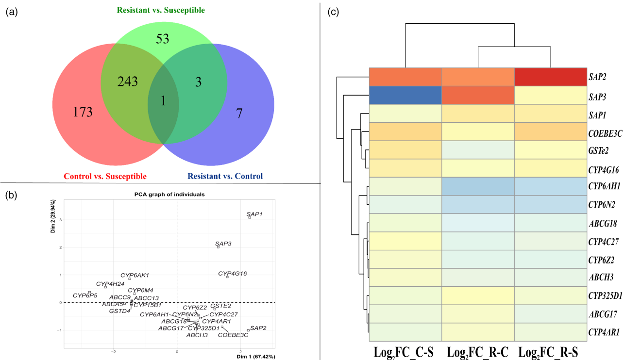
FIGURE 2 Differential gene expression analysis. (a) Venn diagram showing the number of common and specific differentially expressed genes for each comparison between Gounougou and Ngousso. (b) Principal component analysis (PCA) plot showing the most individuals contributing resistant genes involved in the plan of construction. The labelled individuals are those with higher contribution to the plane construction. (c) pHeatmap showing relative expression of the potential first 15 detoxification genes differentially expressed between different comparisons at p -value < 0.05 and \log_2FC > 2 .
