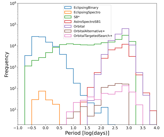
Fig. 2. Number of solutions for each solution type in the nss_two_body_orbit table as a function of period.
