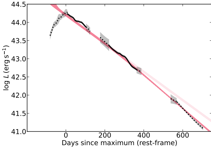
Fig. 23. The bolometric light curve of SN 2018ibb from 1800 to 14 300 Å (rest-frame) and light-curve fits to the fading light curve using the Katz et al. (2013) method. The entire fading light curve from up to 706 days after peak is fully consistent with being powered 24–35 M_{\odot} of ^{56}\text{Ni} (dark red), suggesting that SN 2018ibb could be a pair-instability supernova. At about 300 days after peak (i.e. \geq 400 days after the explosion), the \gamma -ray trapping decreases with time. The loss of trapping is indicated by the difference between the light-red (100% trapping) and dark-red ( <100\% trapping) curves.
