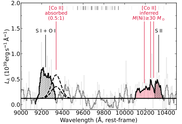
Fig. 29. Zoom-in of the region from 9000 \text{\AA} to 10500 \text{\AA} at t_{\text{max}}+377.5 days. Cobalt has its strongest feature at 1.025 \mu\text{m} . Its tentative detection translates to ^{56}\text{Ni} mass of \gtrsim 30 M_{\odot} , consistent with the light curve modelling. The second strongest cobalt feature is at 9340 \text{\AA} . Its location is indicated by a fiducial Gaussian centred 9340 \text{\AA} . Its integrated luminosity is expected to be between 50 and 100% of [Co II] \lambda 1.025 \mu\text{m} . The absence of [Co II] \lambda 9340 is not an argument against the discovery of [Co II] \lambda 1.025 \mu\text{m} (see Sect. 5.2.5 for details). Lines from other elements that could blend with the [Co II] lines are marked. Regions of strong atmospheric absorption are indicated by vertical bars at the top of the figure.
