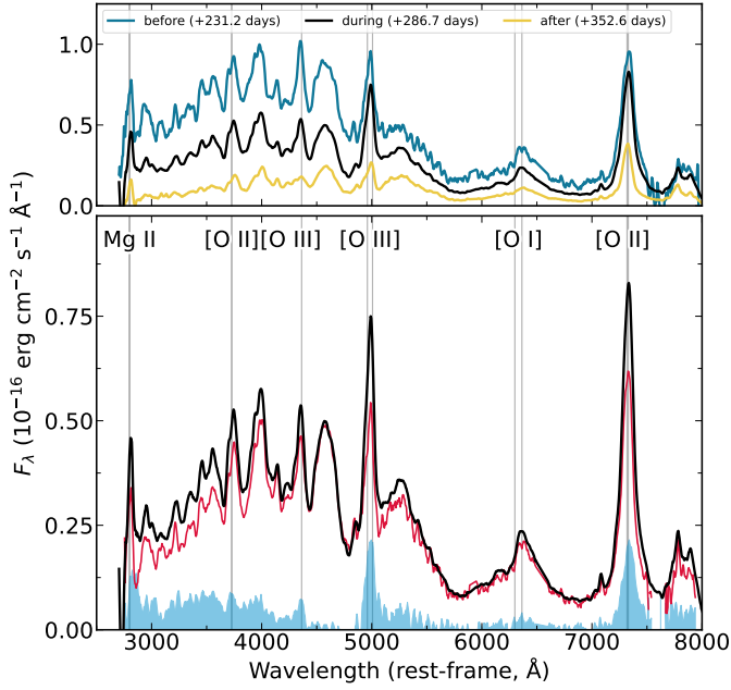
Fig. 13. Impact of the light curve bump between t_{\max}+240 and t_{\max}+340 days on the SN spectrum at t_{\max}+286.7 days. Top: The spectra before, during and after the light curve bump. Bottom: The observed spectrum at t_{\max}+286.7 days ( \approx 13 days before the peak of the bump) is shown in black. We estimate the “bump-free” spectrum of SN 2018ibb at t_{\max}+286.7 days (red) based on the spectra obtained before and after the bump. The difference between the observed (black) and interpolated (red) spectra at t_{\max}+286.7 days is shown in blue. It reveals a series of emission lines that can be attributed to [O II] and [O III]. An excess bluewards of 5000 \text{ \AA} is also visible, while no apparent residual can be seen at the location of [O I].
