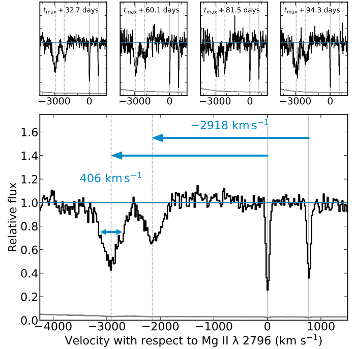
Fig. 12. Normalised X-shooter spectra from t_{\max}+32.7 days to t_{\max}+94.3 days (top panels) and their inverse-variance weighted co-added spectrum (bottom panel). The individual and stacked spectra show barely resolved, narrow absorption lines from the host ISM (marked by the solid vertical lines). In addition, a blue-shifted (2918 km s ^{-1} ) absorption line system is visible (marked by the dashed vertical lines). The FWHMs of the blue-shifted component are 406 km s ^{-1} , significantly larger than the ISM lines but significantly smaller than the SN lines. This blue-shifted absorption-line system is connected with a shell of circumstellar material expelled by the progenitor star shortly before the explosion. No significant evolution in the position or shape of the absorption lines can be seen in the individual spectra (upper panels). The error spectrum is shown in grey.
