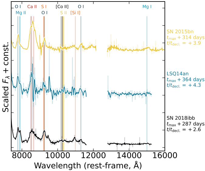
Fig. 35. Late-time NIR spectra of SN 2018ibb and the slow-evolving SLSNe LSQ14an and SN 2015bn. The strongest features are labelled. SN 2018ibb is the only SLSN that shows cobalt in emission, which has its strongest optical-NIR feature at 1.025 \mu\text{m} . Its luminosity translates to a nickel mass of \gtrsim 30 M_{\odot} , consistent with the light curve modelling. All spectra are scaled so that O I \lambda 7773 has the same amplitude in all objects. Regions of strong atmospheric absorption are cropped.
