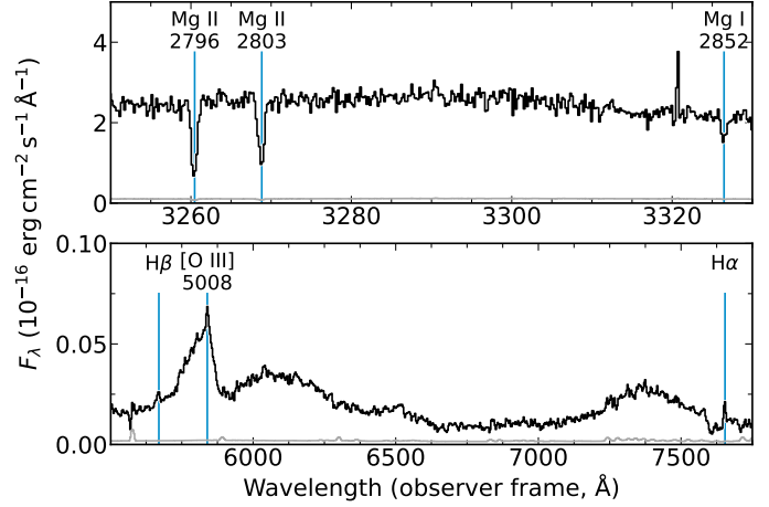
Fig. 2. Galaxy absorption and emission lines at a common redshift of z = 0.166 in the supernova spectra at t_{\max}+32.7 days (top) and at t_{\max}+565.3 days (bottom). The error spectrum of each epoch is shown in grey.
