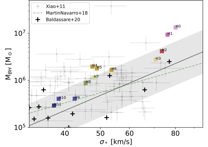
Fig. 2. BH mass versus stellar velocity dispersion ( \sigma_{\star} ) relation for our simulated dwarfs, which are indicated as coloured squares. The velocity dispersion of the stellar component has been measured inside 0.5R_{\text{eff}} for each galaxy. Observations from Xiao et al. (2011) are marked by grey points with error bars, with a 0.2 dex scatter as a grey-shaded area. Observations from Baldassare et al. (2020) are marked by black crosses. The green line shows the Martín-Navarro & Mezcua (2018) observational relation obtained for low-mass Seyfert 1 galaxies. All of our simulated galaxies follow fairly well current existing observational relations between the mass of the central SMBH and the velocity dispersion of the galaxy's stellar component.
