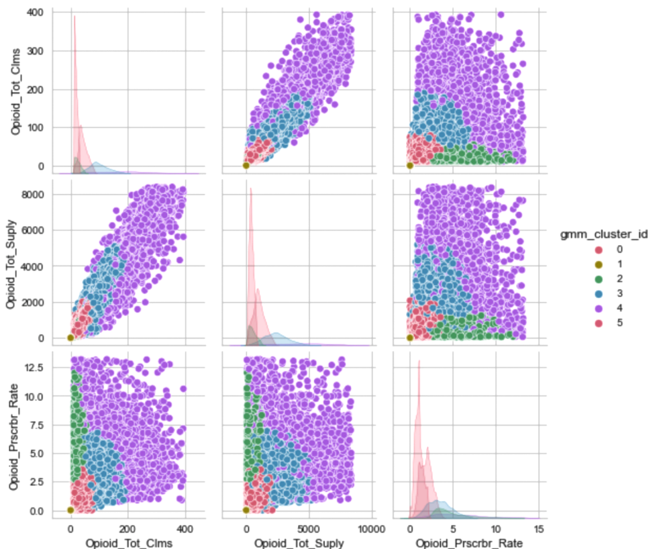
Fig. 5. Pair plot to visualize GMM clustering on the projected data.
