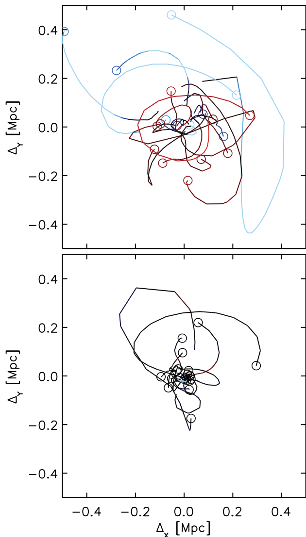
Figure 7. Relative displacement between matched pairs of satellite subhaloes with final masses of \sim 10^{10} M_{\odot} , for pairs with mass ratios that deviate from the median by more than 2\sigma (top panel), or by less than 10 per cent (bottom panel). The circles show the present displacement, while the traces show the evolution from z = 1.5 , coloured according to the mass ratio: black for mass ratios close to the median, red (blue) if the mass in GIMIC is higher (lower) than the median at the time. While most pairs of subhaloes in the bottom panel evolve along similar paths, those in the top panel show more divergent histories, linking the increased scatter among satellites in Fig. 6 to their more chaotic orbits.
