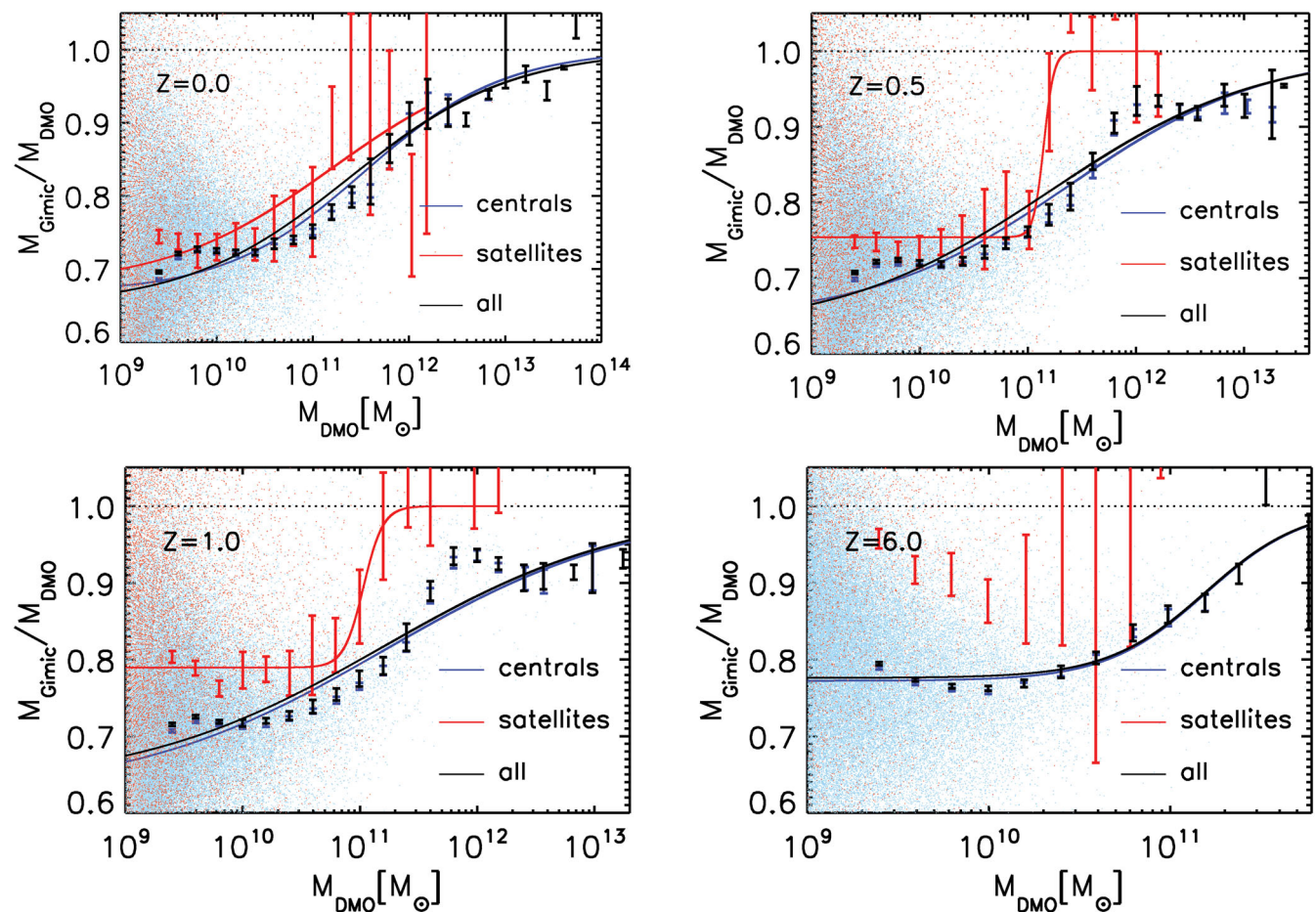
Figure A1. Ratio of subhalo masses between the GIMIC and DMO simulations for matched pairs of subhaloes at different redshift. The error bars indicate the estimate of the median and its error for centrals (blue), satellites (red) and all subhaloes (black), while the lines show the corresponding best fits to equation (2), with coefficients listed in Table A1.
