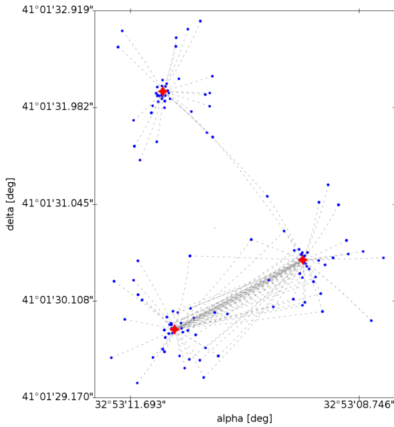
Fig. 16. Example of a match candidate group; in this case comprising three catalogue sources and about 180 observations. Blue dots correspond to observations, red dots are sources, and the dashed lines represent the match candidate source links.
