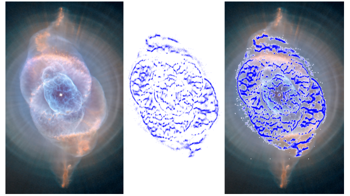
Fig. 14. Cat's Eye Planetary Nebula (NGC 6543) observed with the Hubble Space Telescope (left image) and as Gaia detections (the 84 000 blue points in middle and right images) (Credit: Photo: NASA/ESA/HEIC/The Hubble Heritage Team/STScI/AURA).
