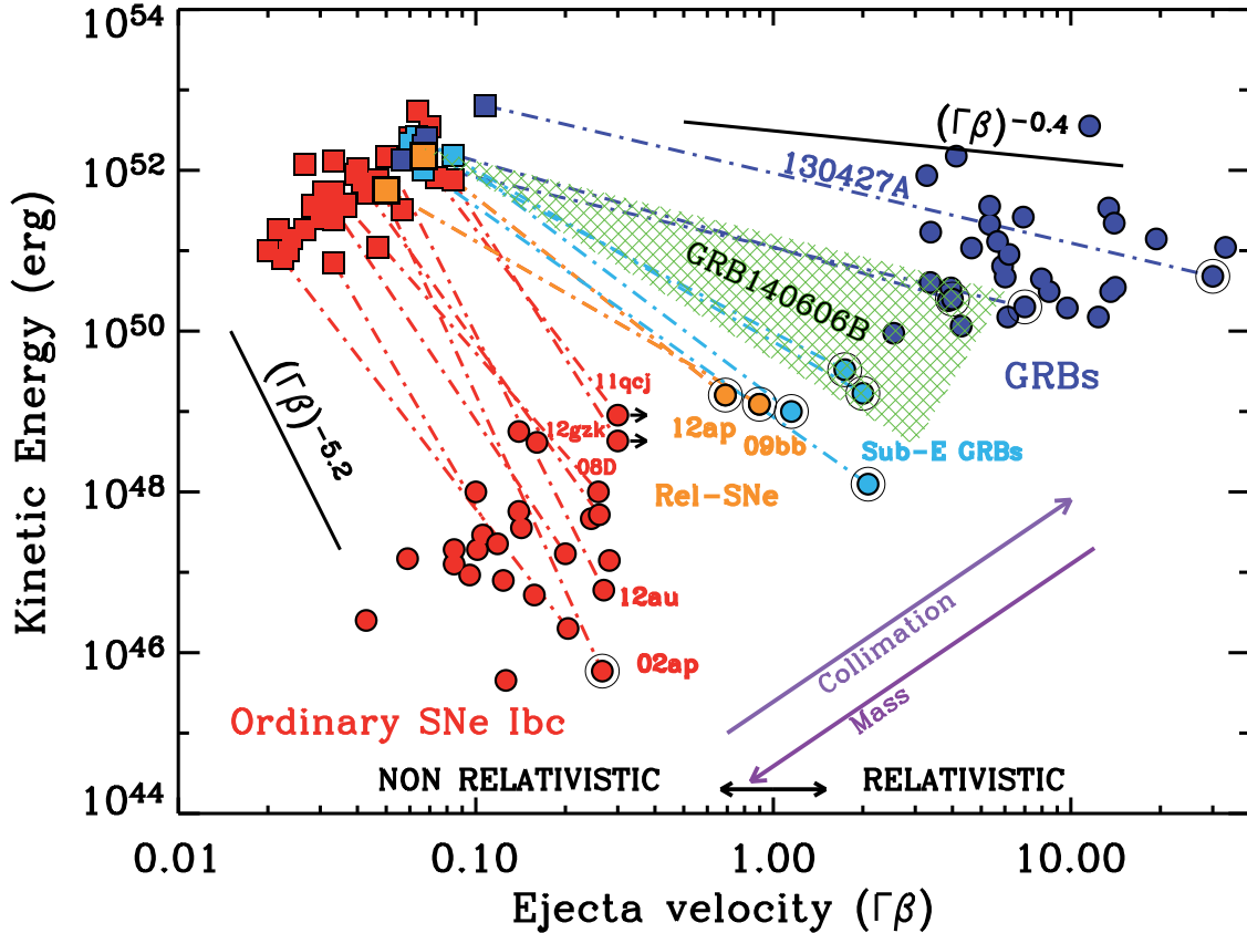
Figure 13. The position of GRB 140606B in the E_K - \Gamma\beta plane. Ordinary SNe Ibc are shown in red, IIGRBs are shown in light blue, relativistic SNe IcbL in orange, and jetted-GRBs in dark blue. Data presented here are from Margutti et al. (2014) and references therein. Squares and circles are used for the slow-moving and the fast-moving ejecta, respectively, as determined from modelling of optical and radio observations of the respective events. Open black circles identify explosions with broad lines in their optical spectra. The velocity of the fast-moving ejecta was computed for t-t_0 = 1 d (rest frame). The black solid lines correspond to ejecta kinetic energy profiles of a purely hydrodynamical explosion E_K \propto (\Gamma\beta)^{-5.2} (Sakurai 1960; Matzner & McKee 1999; Tan, Matzner & McKee 2001), explosions that powered by a short-lived central engine (i.e. an SBO-GRB or a relativistic IcbL SN such as SNe 2009bb and 2012ap; E_K \propto (\Gamma\beta)^{-2.4} ), and those arising from a long-lived central engine (i.e. a jetted-GRB; E_K \propto (\Gamma\beta)^{-0.4} ; Lazzati et al. 2012). The high-energy, relativistic properties of GRB 140606B have been determined using its value of E_{\gamma, \text{iso}} and estimates for its expected \gamma -ray efficiency and an upper-limit to its opening angle as constrained by observations of its optical LC. Despite our conservative estimates of these properties, it is seen that GRB 140606B occupies an intermediate region between SBO-GRBs and jetted-GRBs, and cannot be unambiguously classified as either one type.
