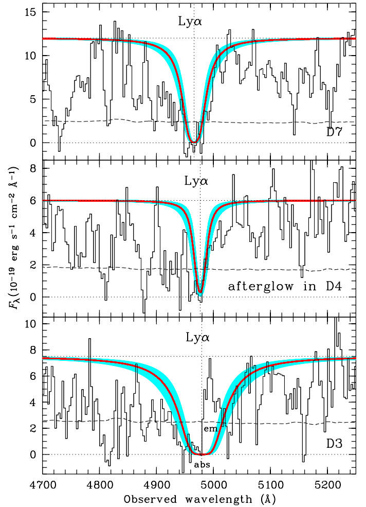
Fig. 5. Fit of the intervening Ly \alpha absorption features towards galaxy D7 ( z_{\text{abs}} = 3.085 ; \log N(\text{H I}) = 20.7 \pm 0.2 ) and towards GRB 070721B ( z_{\text{abs}} = 3.0939 ; \log N(\text{H I}) = 20.1 \pm 0.3 ), and the Ly \alpha absorption feature in the DLA galaxy D3 ( z_{\text{abs}} = 3.096 ; \log N(\text{H I}) = 21.3 \pm 0.2 ). The fit of D3 nicely shows the Ly \alpha emission in the red part of the trough. The afterglow spectrum (D4) was acquired with VLT/FORS2, while the displayed spectra of D3 and D7 were extracted from the VLT/FORS1 data. The fit is shown with a solid line, while 1\sigma errors are displayed with the shaded region.
