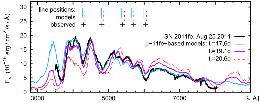
Figure 7. Early-time models for SN 2011fe based on the \rho -11fe density profile, assuming different rise-times t_r between 17.6 d and 20.6 d. The optimum rise-time is determined comparing the positions of prominent features in the optical between observed spectrum (black crosses) and models (light blue/grey, solid lines for 17.6 d; purple/dark grey, solid lines for 19.1 d; red/dark grey, dotted lines for 20.6 d) – analogous to Fig. 4.
