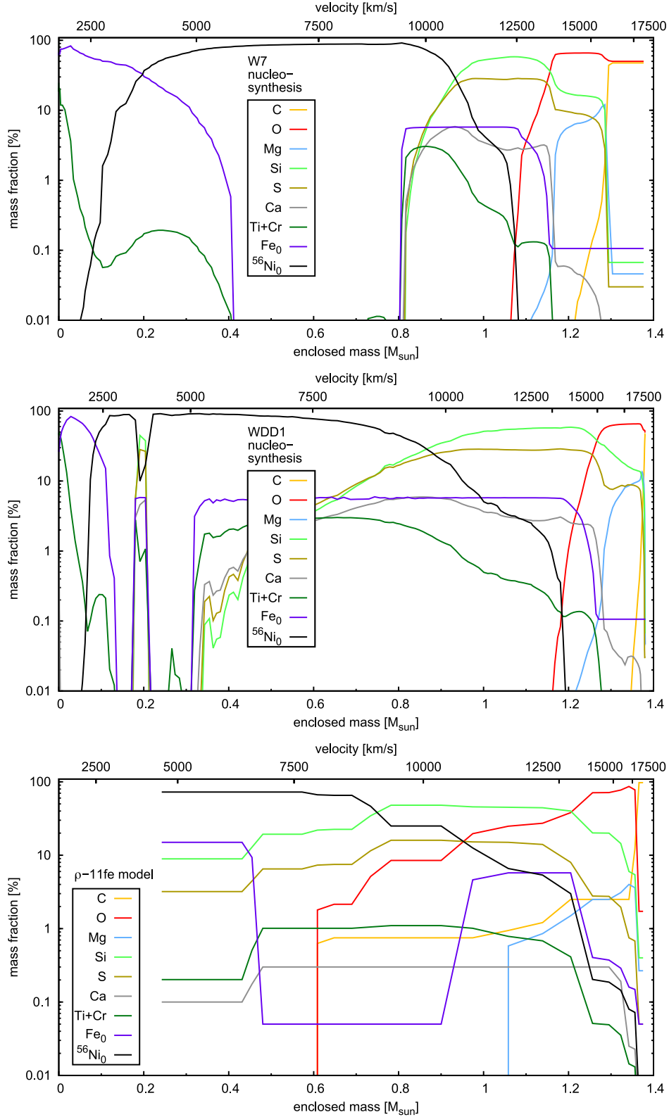
Figure 10. Abundances of W7 and WDD1 nucleosynthesis calculations (Iwamoto et al. 1999, top and middle panel ), plotted in mass space), compared to our tomography based on \rho -11fe ( lower panel ). The Ni/Co/Fe abundances are given in terms of the mass fractions of ^{56}\text{Ni} and stable Fe at t = 0 [ X(^{56}\text{Ni}_0) , X(\text{Fe}_0) ]; stable Ni and Co are present only in traces (few per cent or less by mass) in our model.
