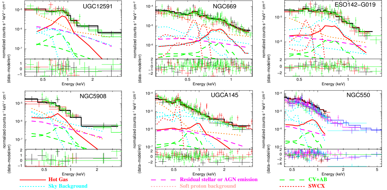
FIG. 3.— Diffuse X-ray spectra extracted from the inner halos of our sample galaxies (white circle or ellipse in Fig. 1). All the spectra have been regrouped to achieve a S/N > 3 . Curves representing different model components are denoted at the bottom of the figure. The plotted data points have been scaled with the effective area of each instrument (MOS-1: black; MOS-2: red; PN: green), so they are consistent with the summation of various model components. There are two observations of NGC 550. Data from the second observation are plotted in blue (MOS-1), cyan (MOS-2), and magenta (PN), respectively.
