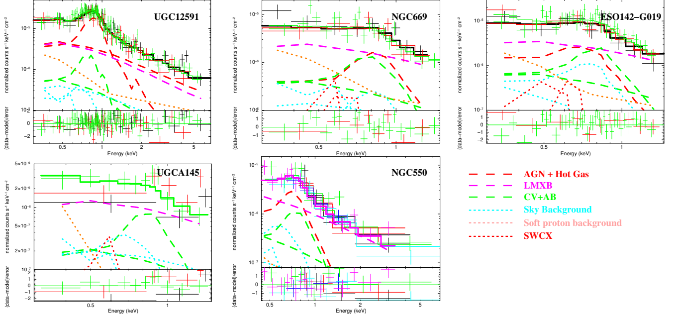
FIG. 16.— AGN spectra extracted from the nuclear region of each galaxy. Curves representing different model components are denoted in the lower right panel. Data points and their scalings are the same as in Fig. 3.
