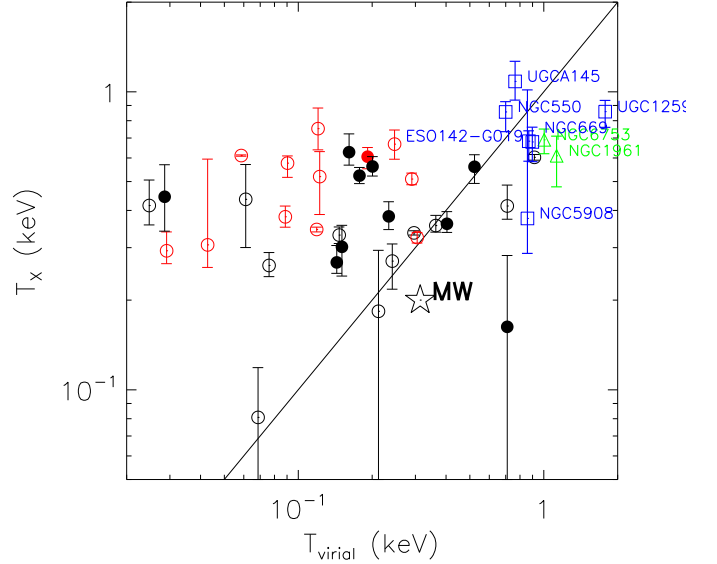
FIG. 7.— Hot gas temperature ( T_X ) measured within the spectral analysis region v.s. the virial temperature of the galaxies ( T_{\text{virial}} ) estimated from their rotation velocity ( v_{\text{rot}} ). Symbols are the same as in Fig. 4. The solid line indicates where T_X = T_{\text{virial}} .
