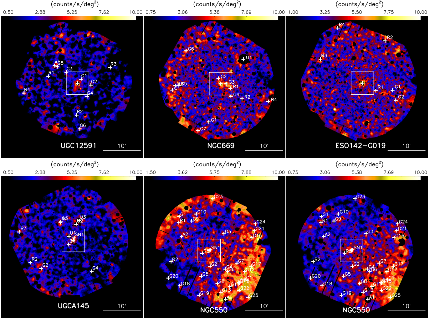
FIG. 14.— Point source removed, soft proton and quiescent particle background subtracted, exposure corrected, and adaptively smoothed 0.5-1.25 keV XMM-Newton EPIC (MOS-1+MOS-2+PN) image of the CGM-MASS galaxies and the surrounding area (a similar image of NGC 5908 is presented in Paper I). The color bar in counts \text{s}^{-1} \text{deg}^{-2} is marked on top of the images. The exposure maps of different instruments are scaled to MOS-2 with the medium filter before the mosaicing. Cross identified sources are marked with pluses, which are also listed in Table 6. The white box in each panel marks the central 6' \times 6' region, the close-up of which is shown in Fig. 1. The last two panels are for different observations of NGC 550, which are separated by two days (ObsID 0741300501 and 0741300601; Table 5).
