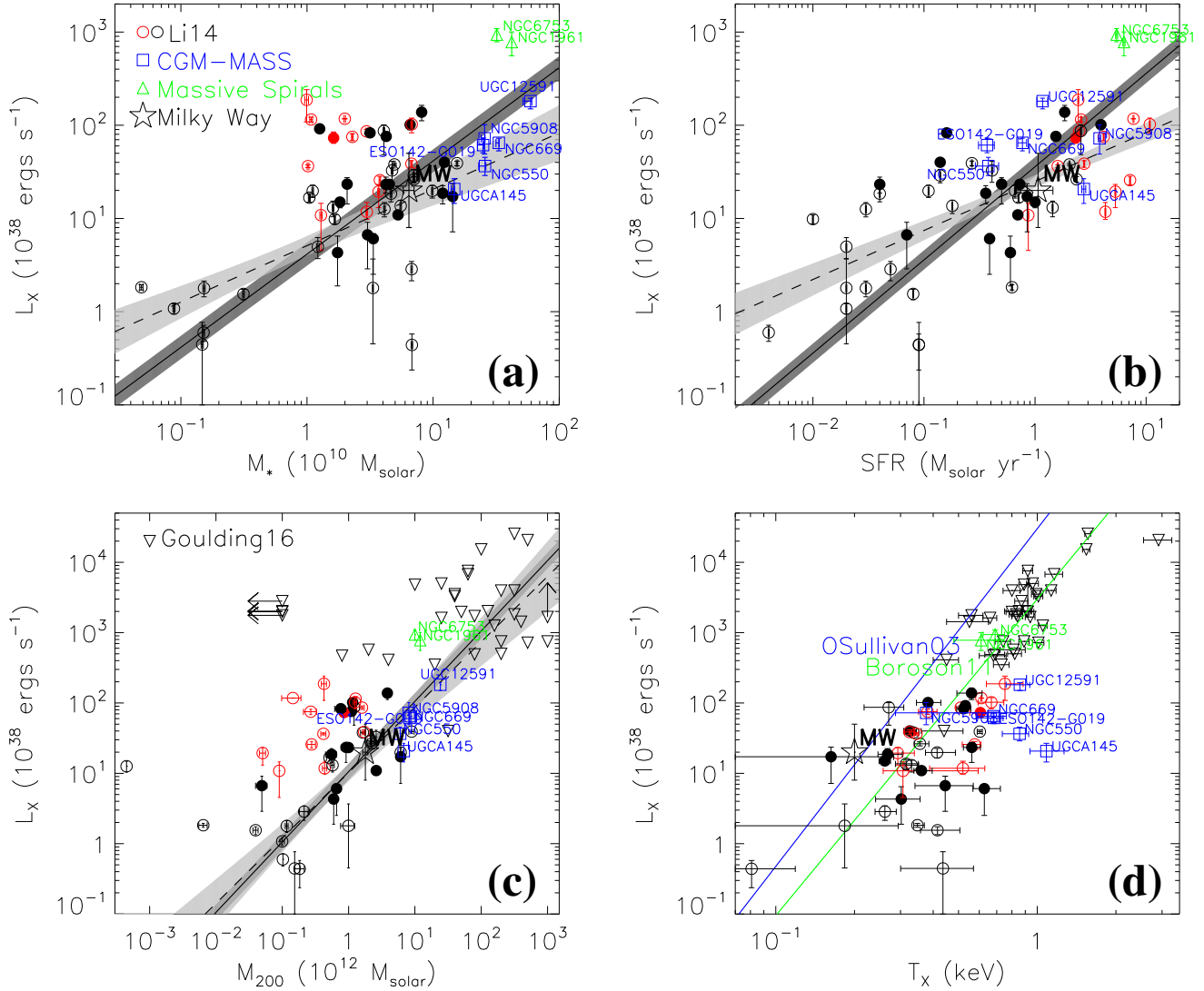
FIG. 4.— X-ray scaling relations of the 0.5-2 keV luminosity of the hot gas ( L_X ) measured in r < 0.1r_{200} v.s. various galaxy properties: (a) stellar mass ( M_* ); (b) SFR; (c) dark matter halo mass ( M_{200} ) estimated from the rotation velocity v_{\text{rot}} ; (d) hot gas temperature ( T_X ) measured within the spectral analysis region. Symbols representing data from various samples are denoted in panels (a) and (c). The homogenization of these data are discussed in detail in §3. Names of the CGM-MASS galaxies, other massive spiral galaxies, and the Milky Way (MW) are denoted beside the data points. The circles (both filled and open) represent the nearby highly-inclined disk galaxies studied in Li & Wang (2013a,b); Li et al. (2014). Red/black circles represent starburst/non-starburst galaxies, while open/filled circles are field/clustered galaxies, respectively. We also include Chandra measurements of the MASSIVE early-type galaxy sample (Goulding et al. 2016) for comparison in panels (c) and (d) (downward triangles). The blue and green solid lines in panel (d) are the best-fit T_X - L_X relations from the high- and low-mass elliptical galaxy samples of O’Sullivan et al. (2003) and Boroson et al. (2011), respectively. The black solid lines in panels (a-c) are linear fit to different subsamples of Li & Wang (2013a)’s sample [non-starburst field galaxies in (a); the whole sample in (b); non-starburst field galaxies with v_{\text{rot}} > 50 \text{ km s}^{-1} in (c)] and the dark shaded region represents the 1-\sigma confidence range. The black dashed line and light shaded regions represent non-linear fit (power law with slope set free) and 1-\sigma confidence range of the same subsamples.
