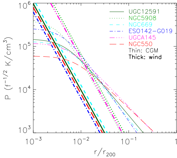
FIG. 12.— Hot gas thermal pressure profile (thin curves) calculated with Equ. 4 and parameters listed in Tables 2 and 3. We also include the thermal pressure of a star formation driven wind blown bubble for comparison (thick curves; Veilleux et al. 2005).
