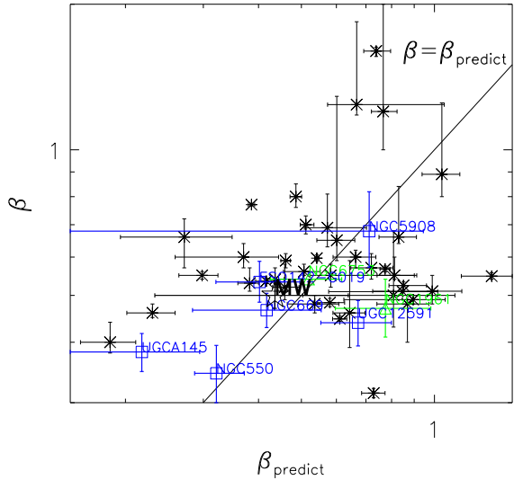
FIG. 10.— The measured and predicted \beta index of the \beta function describing the radial intensity profiles of massive spiral galaxies and O’Sullivan et al. (2003)’s X-ray luminous elliptical galaxies. \beta_{\text{predict}} is estimated by assuming a hydrostatic-isothermal model of the hot halo gas (Jones & Forman 1984). See the text for details. Symbols are the same as in Fig. 8. The solid line indicates where \beta = \beta_{\text{predict}} .
