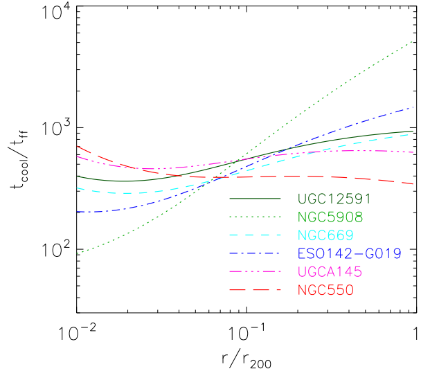
FIG. 11.— Radial profile of t_{\text{cool}}/t_{\text{ff}} of different CGM-MASS galaxies. Note that we have assumed the stellar mass of the galaxy is a mass point, which is only valid at large radii. Therefore, at small radii (typically < 0.1r_{200} ), the real t_{\text{cool}}/t_{\text{ff}} should be smaller than plotted on the figure.
