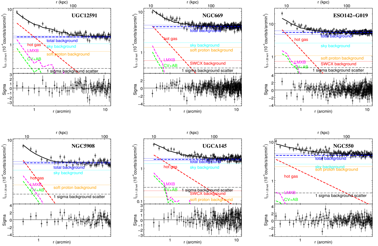
FIG. 2.— Radial intensity profile of the diffuse 0.5-1.25 keV emission around the center of the CGM-MASS galaxies. The upper and lower axes denote the off-center distances in unit of kpc and arcmin, respectively. X-ray bright nuclei of the galaxies are masked off (Fig. 1), so the profiles typically start at r \approx 0.5' . The best-fit model, shown as a thick black solid curve, is comprised of several components: the sky+SP+SWCX background (blue dashed), the LMXB and CV+AB contributions estimated from the K-band intensity profile (magenta and green dashed), and a \beta -function representing the hot gas distribution (red dashed). Statistical plus systematic uncertainties of the best-fit background level are plotted as blue thin dotted lines. For comparison, we also plot the sky (cyan), SP (orange), and SWCX (red; whenever applicable) background components with thin dotted lines, separately. The 1\sigma scatter of the background estimated in radial ranges with flat background is also plotted as a thin dashed black line.
