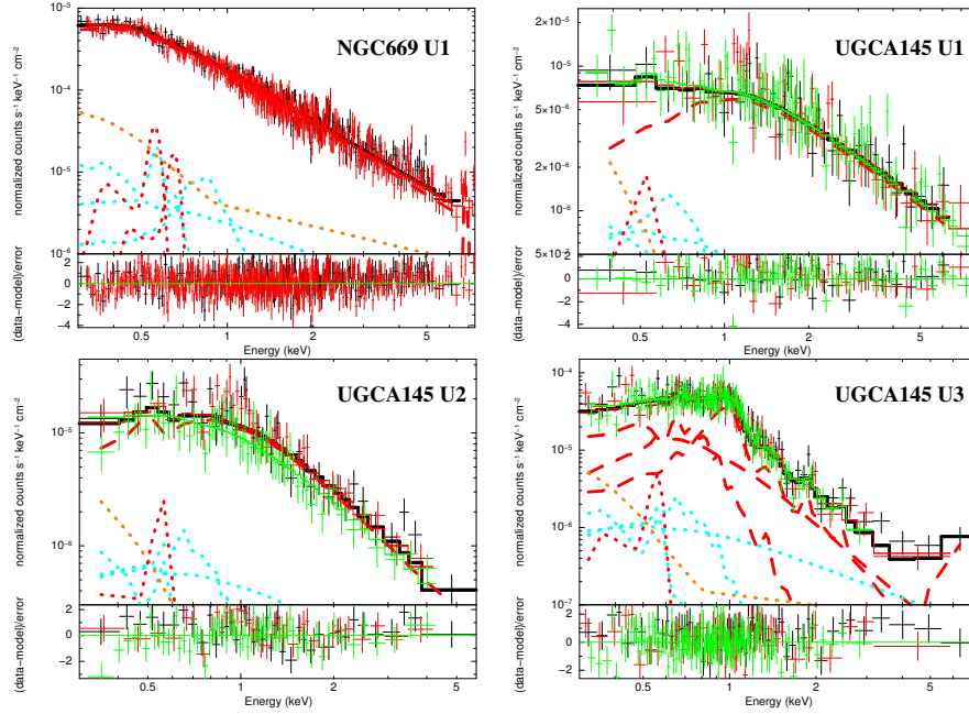
FIG. 17.— XMM-Newton spectra of X-ray bright unidentified point-like sources. Locations of the sources are shown in Fig. 14 and listed in Table 6. Symbols are the same as in Fig. 16. MOS-1 does not cover NGC 669 U1 (due to the removal of noise CCD), so only MOS-2 (black) and PN (red) spectra are shown.
