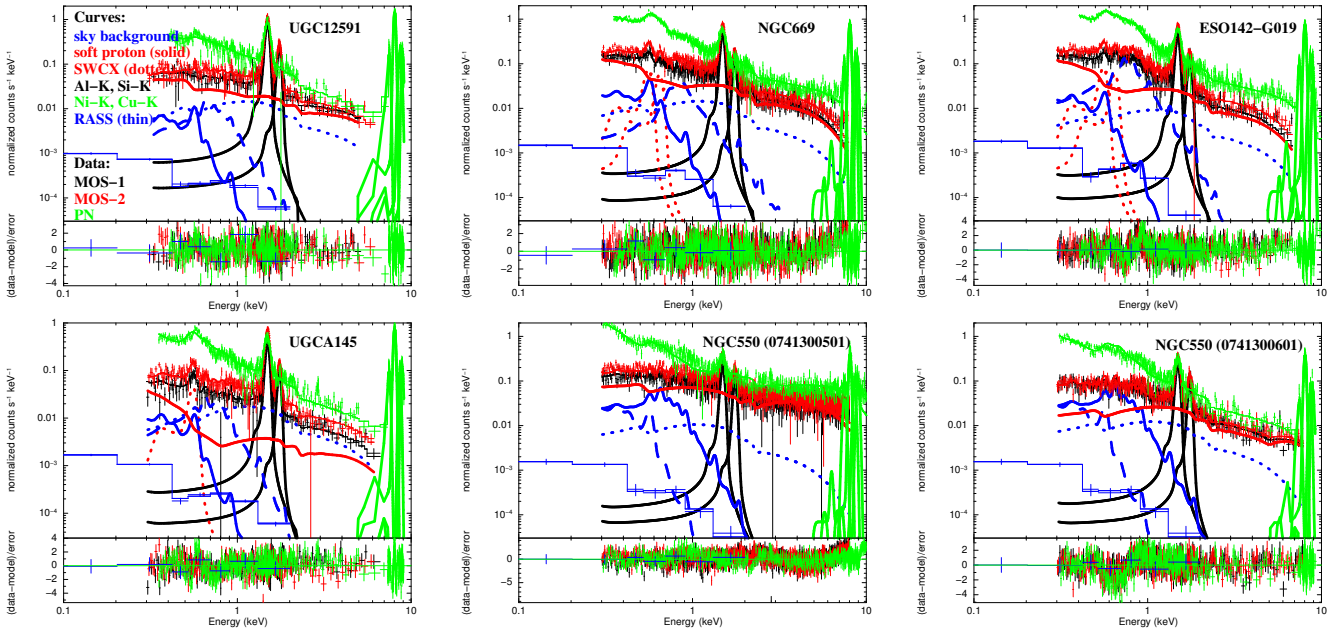
FIG. 13.— Background spectra of the CGM-MASS galaxies extracted from a large enough annulus to exclude the emission associated with the galaxy. We also remove point sources and prominent diffuse X-ray features using the masks shown in Fig. 15. These spectra are similar as the background spectra of NGC 5908 presented in Paper I, but we add a SWCX component for some galaxies. The ROSAT all sky survey (RASS) spectrum extracted from a 0.2^\circ - 1^\circ annulus centered at the galaxy is also included in order to help constraining the sky background (blue data points and thin solid curve). Curves of different model components are scaled to the MOS-1 spectrum, except for the Ni and Cu K\alpha lines, which are scaled to the PN spectrum. Colored data points with error bars are spectra of MOS-1 (black), MOS-2 (red), and PN (green), respectively. Colored curves denote different background model components: sky background including the local hot bubble (blue solid), the Galactic halo (blue dashed), and the distant AGN (blue dotted) components, soft proton (red), SWCX (red dotted), Al- K\alpha and Si- K\alpha instrumental lines (two black gaussian lines), and Ni- K\alpha and Cu- K\alpha lines of PN only (four green gaussian lines). The two observations of NGC 550 are plotted in separated panels.
