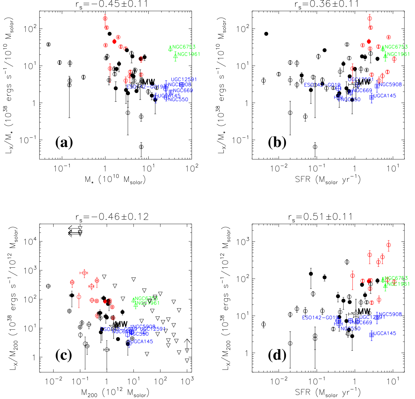
FIG. 5.— Specific X-ray luminosity ( L_X/M_* or L_X/M_{200} ) plotted against other galaxy properties. The Spearman’s rank order correlation coefficient r_s are calculated for all the galaxies plotted in each panel, except for the MASSIVE sample in panel (c) (open downward triangles).
