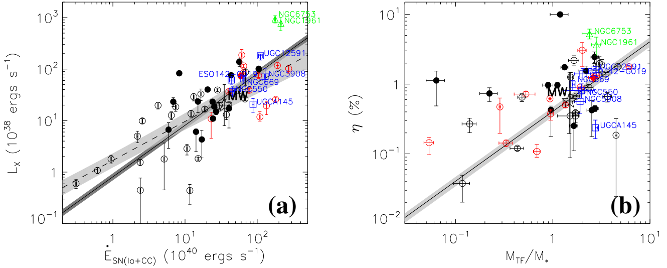
FIG. 9.— (a) L_X measured in r < 0.1r_{200} v.s. the total (Type Ia + core collapsed) SN energy injection rate [ \dot{E}_{\text{SN(Ia+CC)}} ]. (b) The X-ray radiation efficiency [ \eta \equiv L_X/\dot{E}_{\text{SN(Ia+CC)}} ] v.s. the baryonic to stellar mass ratio ( M_{\text{TF}}/M_* ). Symbols are the same as in Fig. 4.
