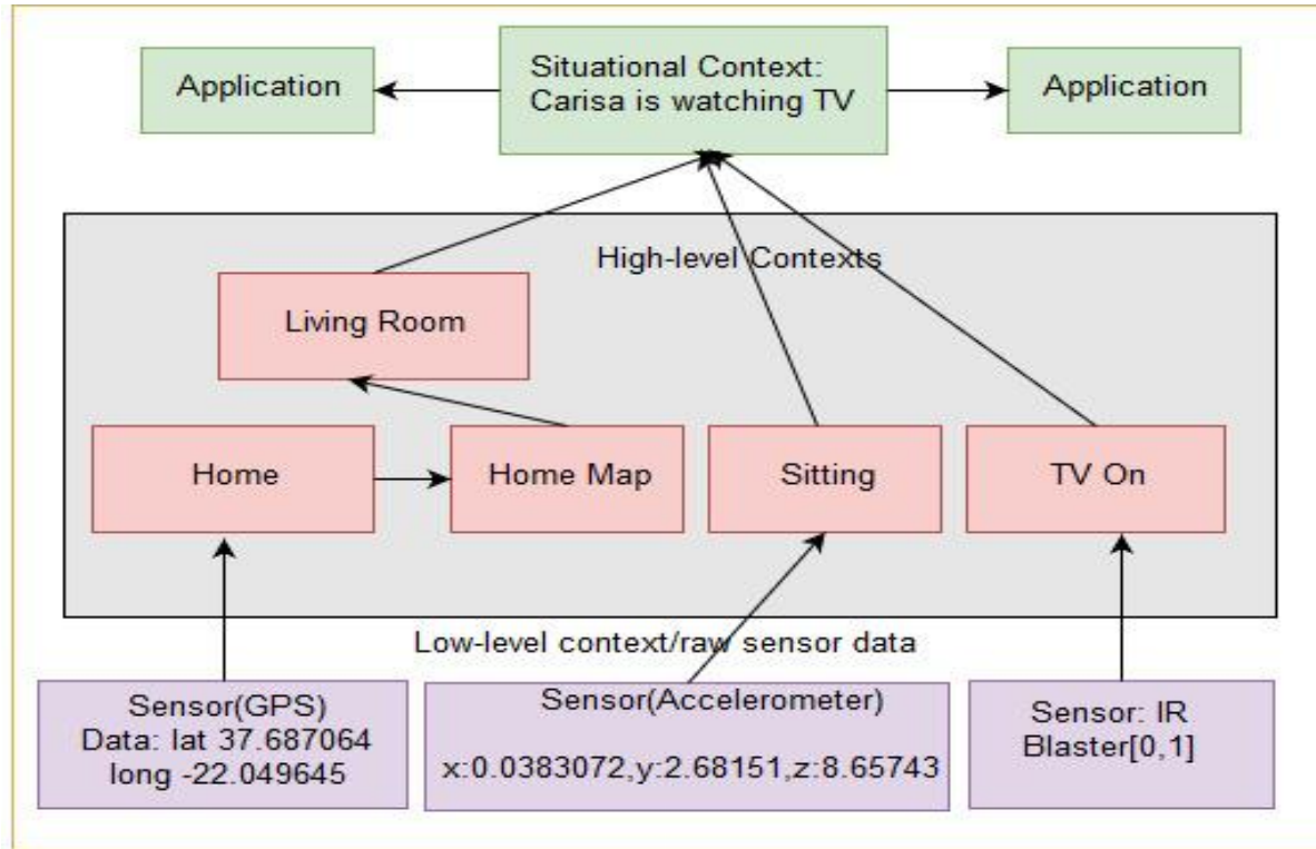
Figure 8: Situational context from High-level context and low-level context data
