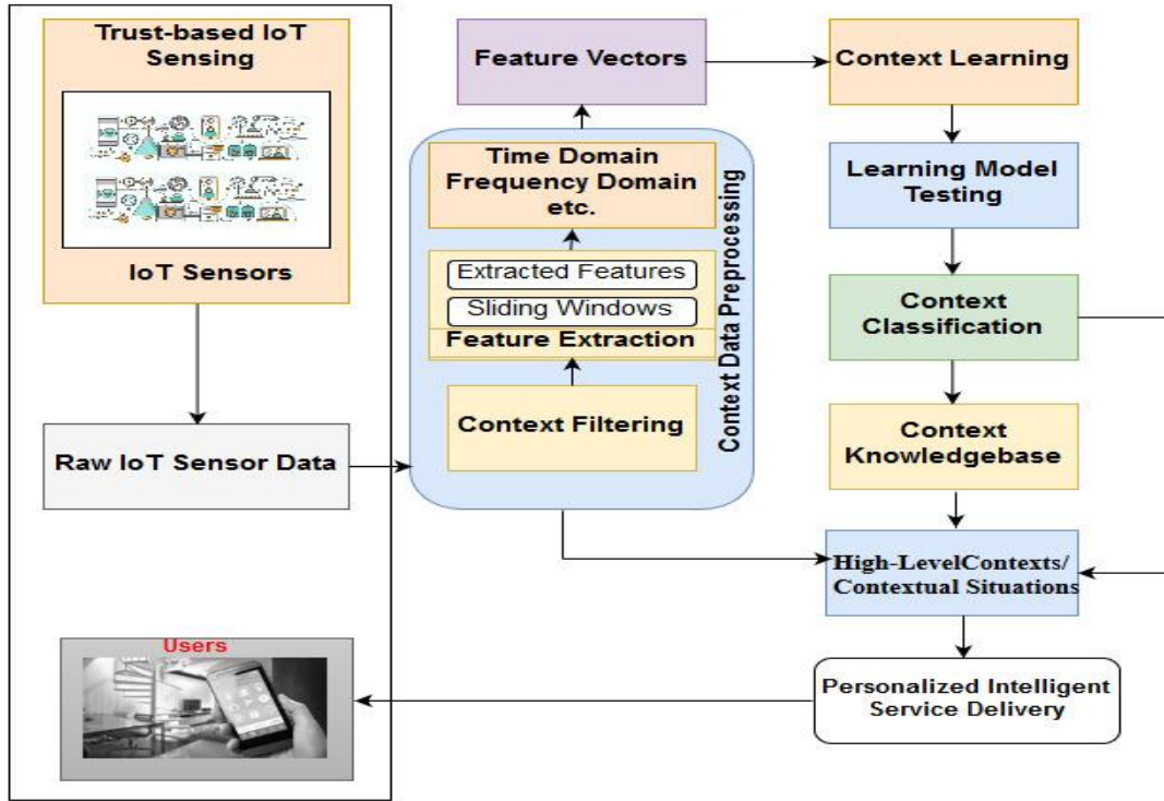
Figure 6: Context Recognition Processes of the proposed Framework
