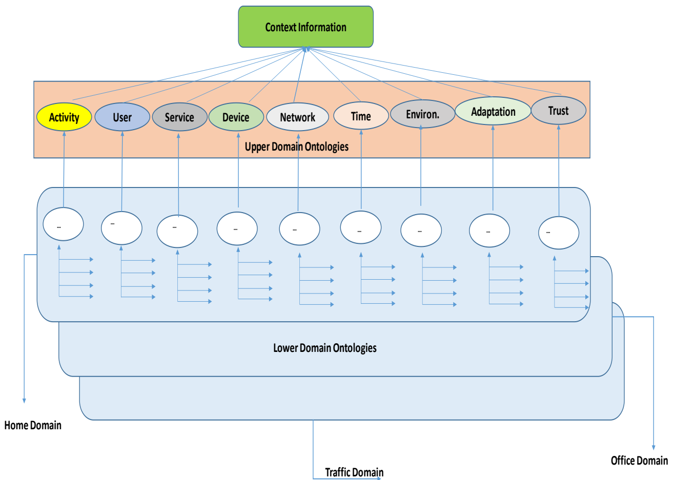
Figure 10: Cognitive Upper and Lower Domain Context Ontology Model
