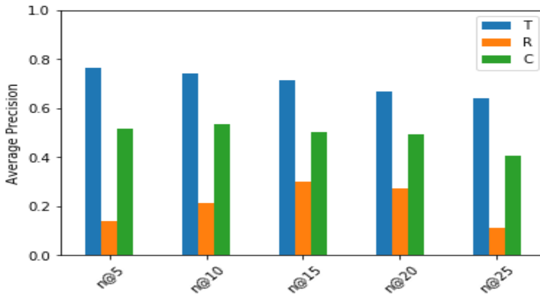
Figure 21: Comparison of Average Precision for Traditional Recommendation (R), Context based Recommendations(C) and Trust based Recommendation ( T)
