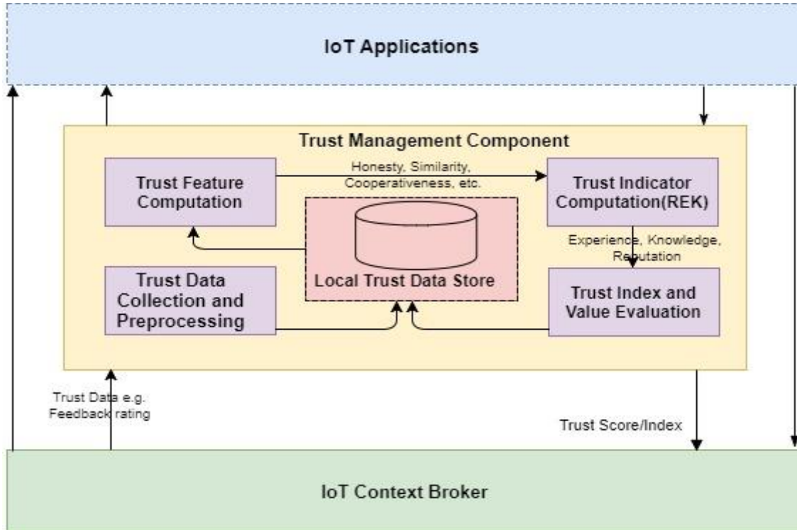
Figure 14: Trust Computation Component.
