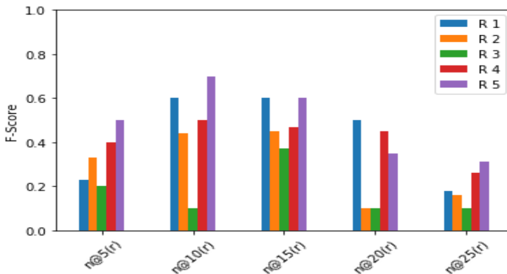
Figure 18: F-Score for non-contextual preferences
