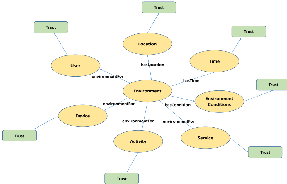
Figure 11: Relationship between the framework ontology concepts and Trust
