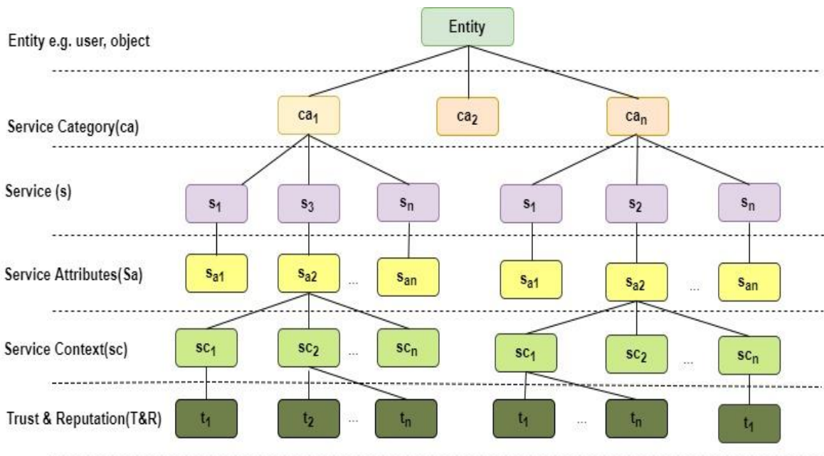
Figure 15: The Preference Model, showing structure and relationships between entities in the profile model.
