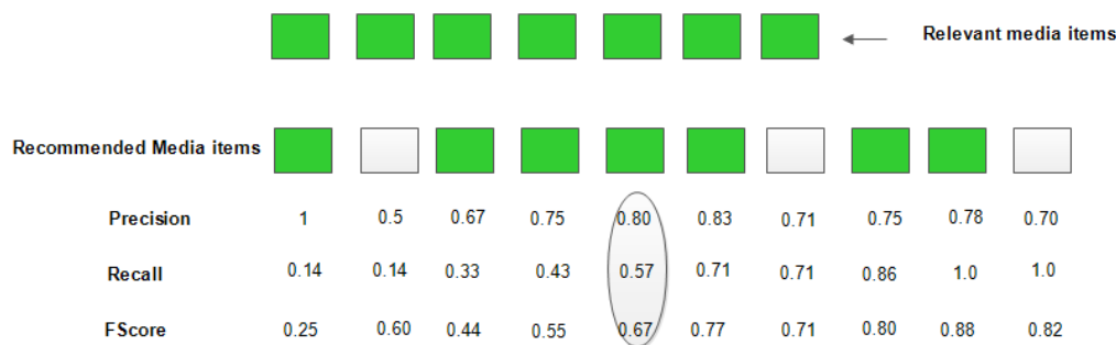
Figure 16—Computing precision, recall and f-score for recommendation system [45]
