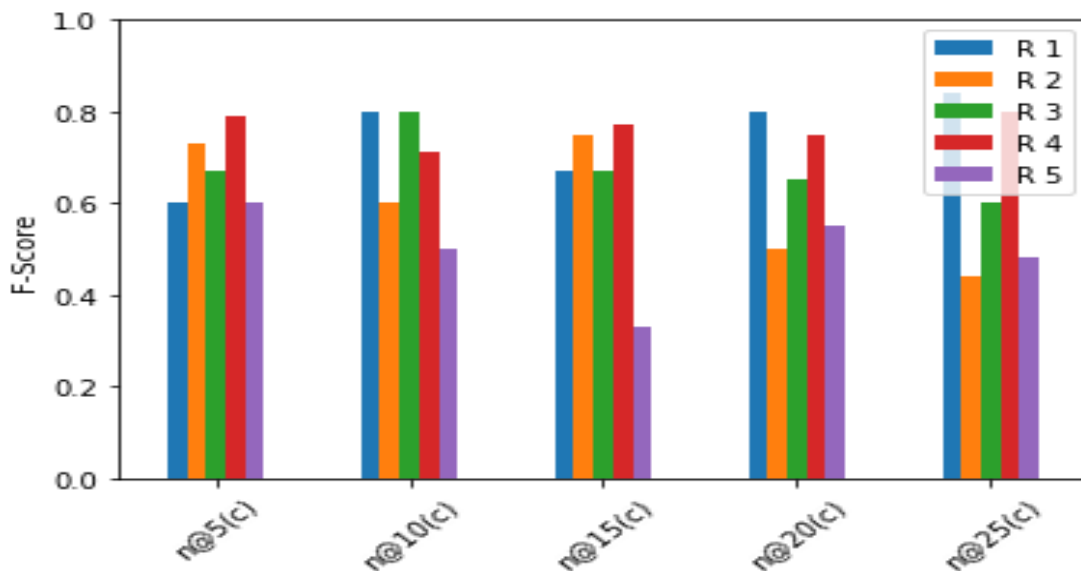
Figure 19: Comparison of F-Score for contextual preferences
