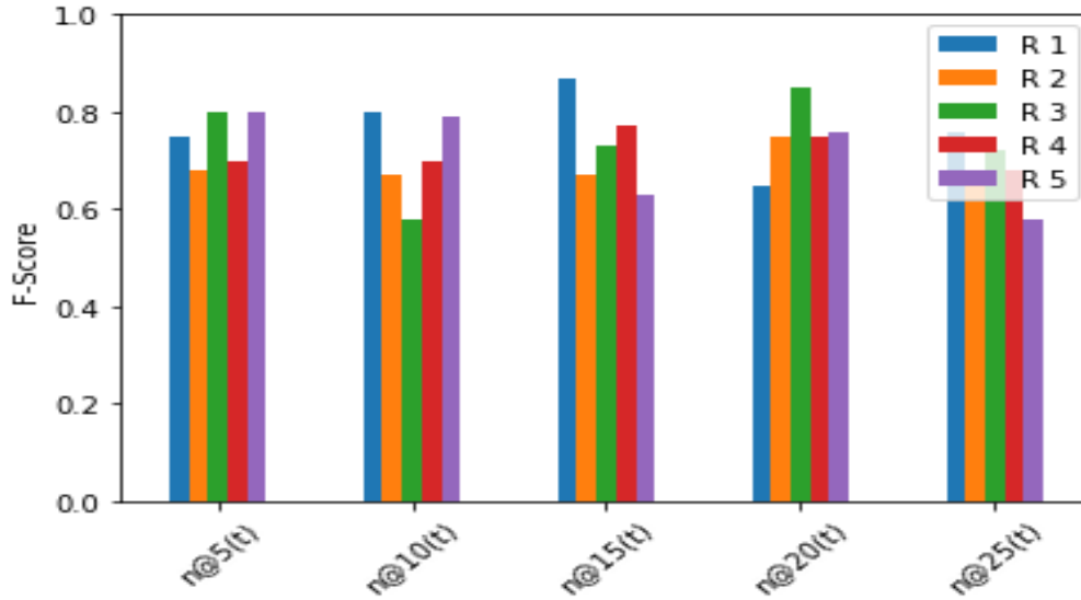
Figure 20: Comparison of F-Scores for preference with trust based contextual preferences
