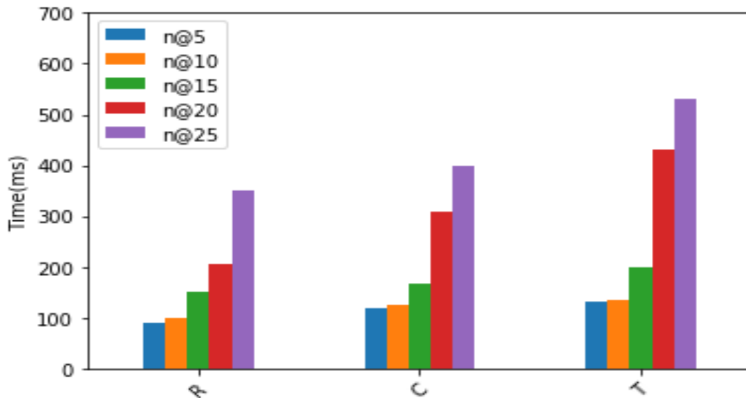
Figure 22: Comparison of time taken by Traditional Recommendation (R), Context based Recommendations(C) and Trust based Recommendation (T) to generate ranked recommendations
