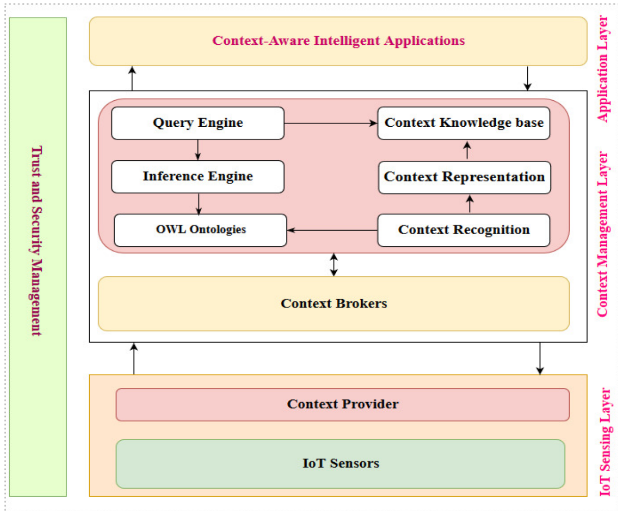
Figure 7: High-level architecture of the proposed cognitive context-awareness, an extension of Figure 6
