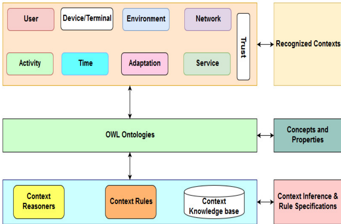
Figure 9: The Framework Inference Model
