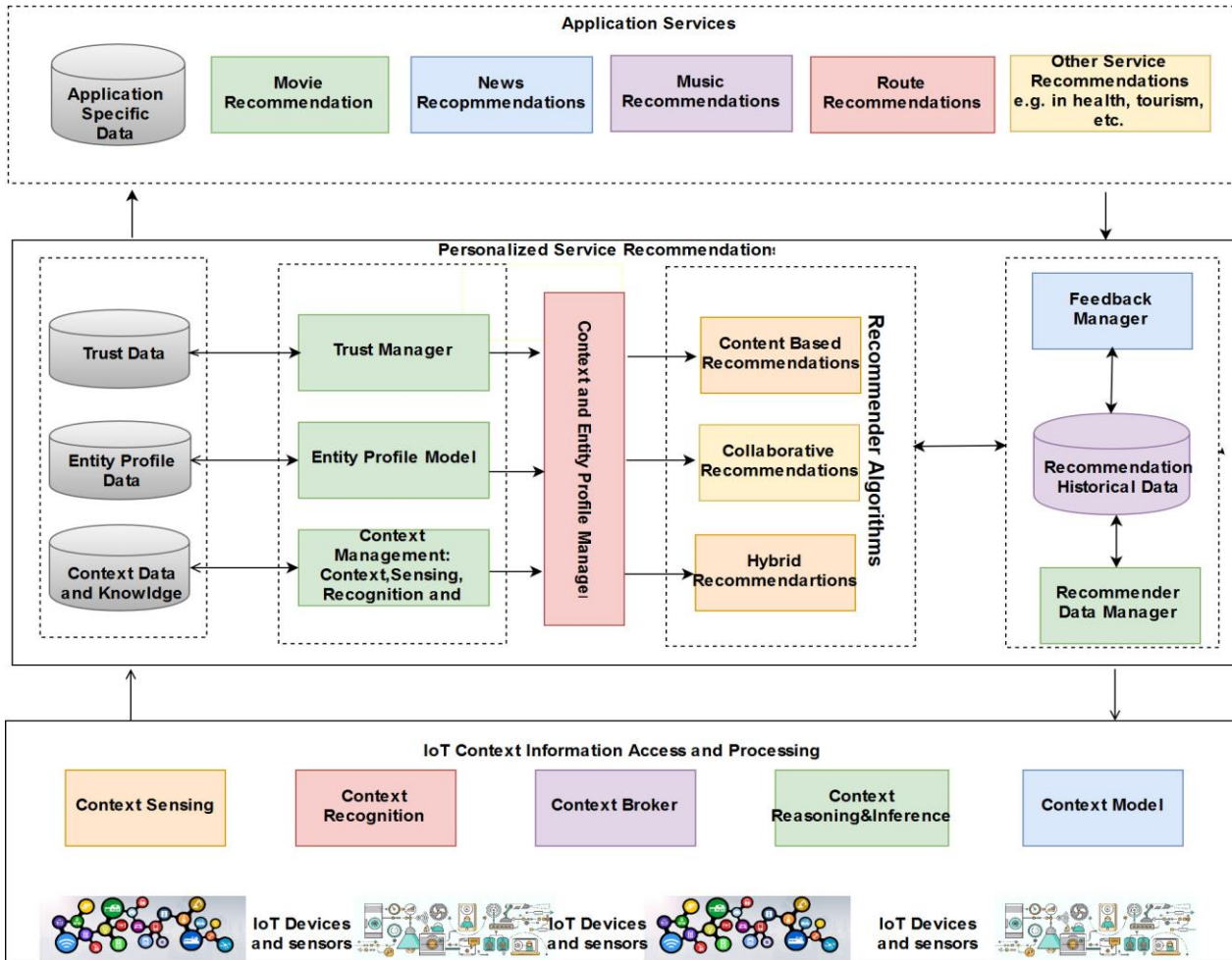
Figure 5: Components of the proposed Trust-based Context-aware Recommendation System
