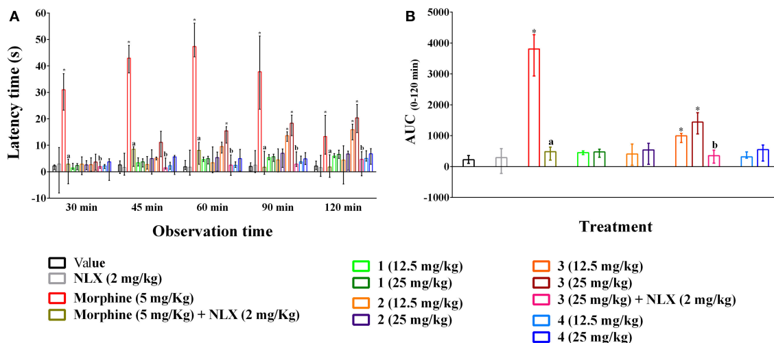
FIGURE 4 | Effect of compounds 1–4 , morphine and pre-treatment of naloxone in tail immersion test. (A) maximal percent of analgesic effect (% MPE) of compounds 1–4 , morphine and antagonist effect of naloxone. (B) area under the curve (AUC 0–120 min ) response of the compounds 1–4 , morphine and pre-treatment of naloxone. Values are presented as median ( n = 6 ) with range (min-max). 1 = 3,3',5,6,7,8-hexamethoxy-4',5'-methylenedioxyflavone; 2 = exotixin; 3 = 6,7,4',5'-dimethylenedioxy-3,5,3'-trimethoxyflavone; 4 = 3,3',4',5,5',8-hexamethoxy-6,7-methylenedioxyflavone, NLX = naloxone. * p < 0.01 , compared to control group. a,b p < 0.01 , compared to morphine (5 mg/kg) and 3 (25 mg/kg) respectively.
