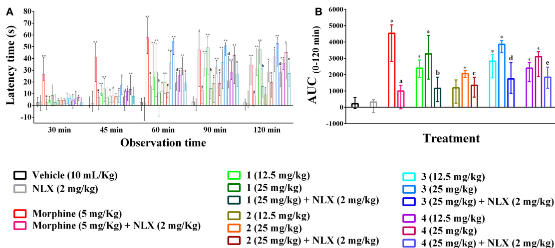
FIGURE 3 | Effect of compounds 1–4 , morphine and pre-treatment of naloxone in hot plate test. (A) Maximal percent of analgesic effect (% MPE) of compounds 1–4 , morphine and antagonist effect of naloxone. (B) Area under the curve (AUC 0–120 min ) response of the compounds 1–4 , morphine and pre-treatment of naloxone. Values are presented as median ( n = 6 ) with range (min-max). 1 = 3,3',5,6,7,8-hexamethoxy-4',5'-methylenedioxyflavone; 2 = exotixin; 3 = 6,7,4',5'-dimethylenedioxy-3,5,3'-trimethoxyflavone; 4 = 3,3',4',5,5',8-hexamethoxy-6,7-methylenedioxyflavone, NLX = naloxone. *, ** p < 0.05 and p < 0.01 , compared to control group, respectively. a,b,c,d,e p < 0.05 , compared to morphine (5 mg/kg), 1 (25 mg/kg), 2 (25 mg/kg), 3 (25 mg/kg), and 4 (25 mg/kg), respectively.
