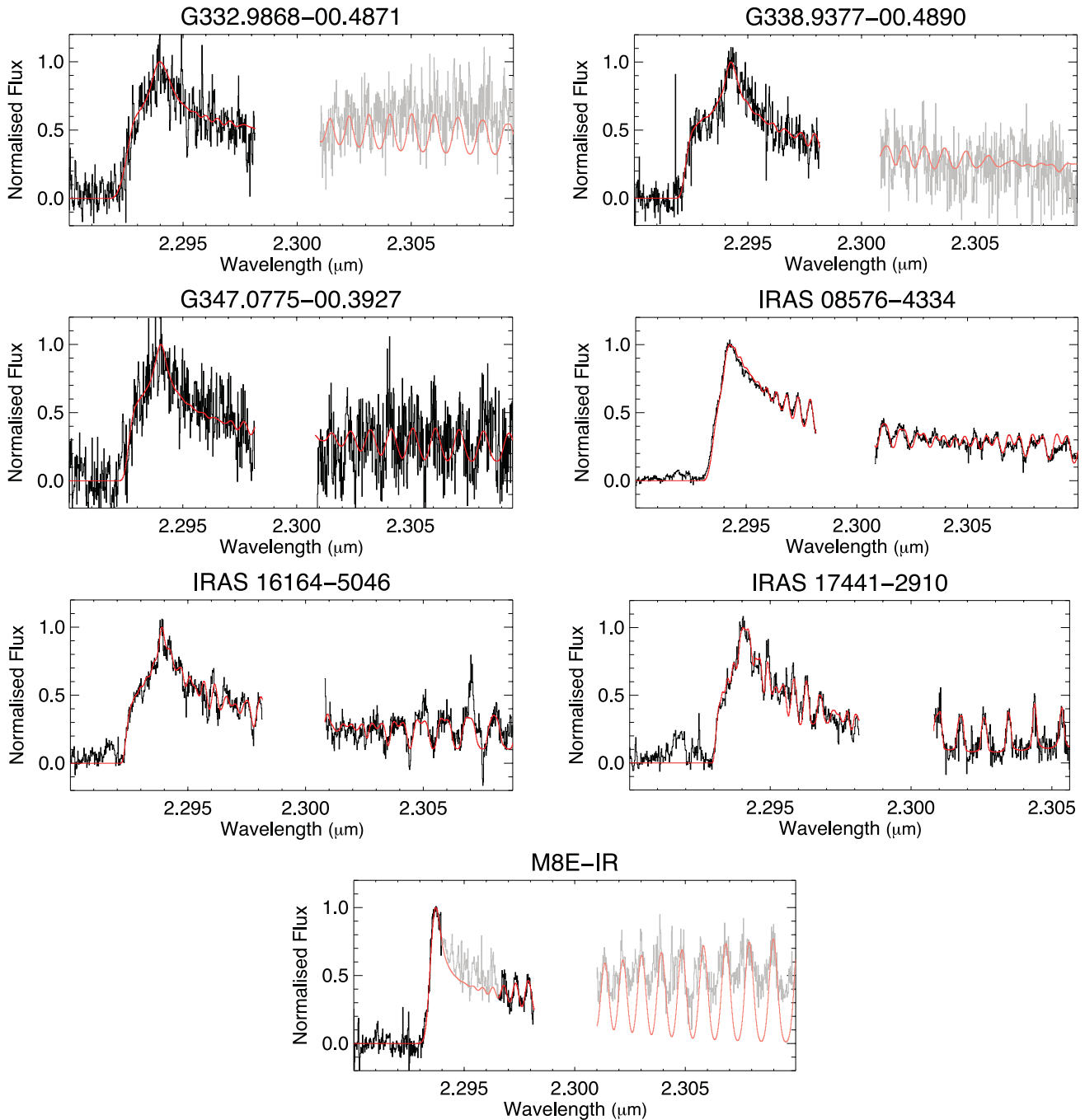
Figure 4. Spectra (black) and model fits (red) to the CO emission of the objects in the sample, using disc Model A. Data that are greyed out are not included in the fitting procedure because of poor quality, but have been included for completeness. The range of fitting for M8E-IR was restricted to obtain a good fit (see Appendix A for full discussion). For IRAS 17441–2910, the portion of the spectrum beyond 2.306 \mu\text{m} was not used because an artificial drop in flux was caused by the detector.
