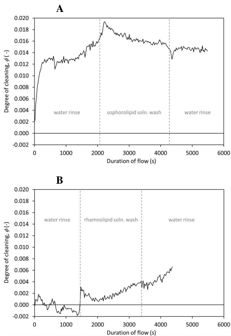
Figure 3. Degree of cleaning over rinse-wash-rinse cycle. A. Sophorolipids 0.4 g/L wash. B. Rhamnolipids 0.4 g/L wash.
