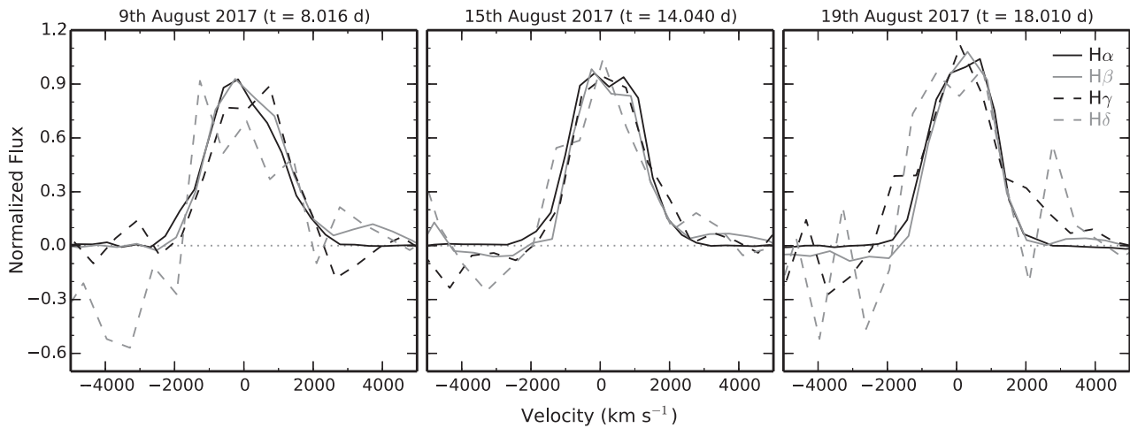
Figure 3. The evolution of the AT2017fvz H \alpha –H \delta emission lines over \sim 18 d post-eruption (normalized to peak flux). The H \delta profile shows tentative evidence for blueshifted absorption ( t = 8.016 d) – a possible P Cygni profile.
