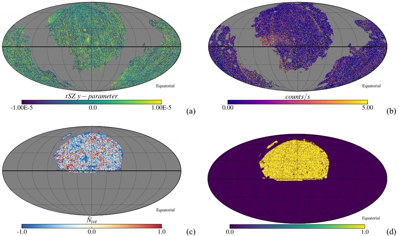
Figure 5. (a) A map of mean-subtracted tSZ y parameter as produced by the MILCA component separation algorithm from Planck 2015 data. Milky Way and point-source masks have been applied (grey regions). The map has also been transformed into equatorial coordinates and rotated so that the region overlapping with SDSS footprint is in the centre. (b) A map of mean-subtracted X-ray flux in count \text{s}^{-1} from RASS. Milky Way and point-source masks have been applied (grey regions). The map has also been transformed into equatorial coordinates and rotated so that the region overlapping with SDSS footprint is in the centre. (c) A map of SPH-smoothed SDSS galaxies in the spectroscopic sample (galaxy overdensity), projected on to the healpix sphere. The final 7849 \text{deg}^2 footprint is as a result of a combination of the Milky Way, point source, and main SDSS footprint coverage. (d) Final mask resulting from the combination of Milky Way, point source, main SDSS footprint, and zero exposure by ROSAT masks. This mask gives a sky fraction of 0.16 and is used in all correlations for respective galaxy samples in this paper. These and other maps will be made publicly available at http://www.astro.ljmu.ac.uk/env_cor/ .
