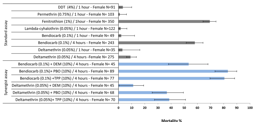
Figure 2. Insecticide susceptibility status of C. quinquefasciatus from Tororo (Uganda). Bioassay results following exposure to WHO insecticide treated papers at standard conditions and effect of insecticide synergists on the susceptibility status. Grey and blue bars represent WHO standard and synergists bioassay, respectively. Error bars represent 95% CI. PBO: piperonyl butoxide, DEM: diethyl maleate, TPP: triphenyl phosphate.
