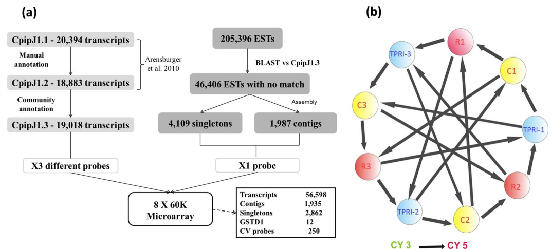
Figure 1. Overview of Culex quinquefasciatus whole-transcriptome analysis. (a) Design of the 8 × 60 K Agilent microarray. CpipJ1: consensus gene set of the automated gene prediction from the C. quinquefasciatus Johannesburg strain genome sequence. EST: expressed sequence tags. GSTD1: Glutathione S transferase D1. CV probe: coefficient of variation. (b) Interwoven hybridization loop design for comparison between bendiocarb exposed and non-exposed Ugandan field-collected mosquitoes and the TPRI susceptible strain. Circles represent pools of 10 females. C: Uganda non-exposed mosquitoes (sympatric control), R: Uganda Resistant mosquitoes, TPRI (Tropical Pesticides Research Institute): C. quinquefasciatus susceptible strain from Tanzania.
