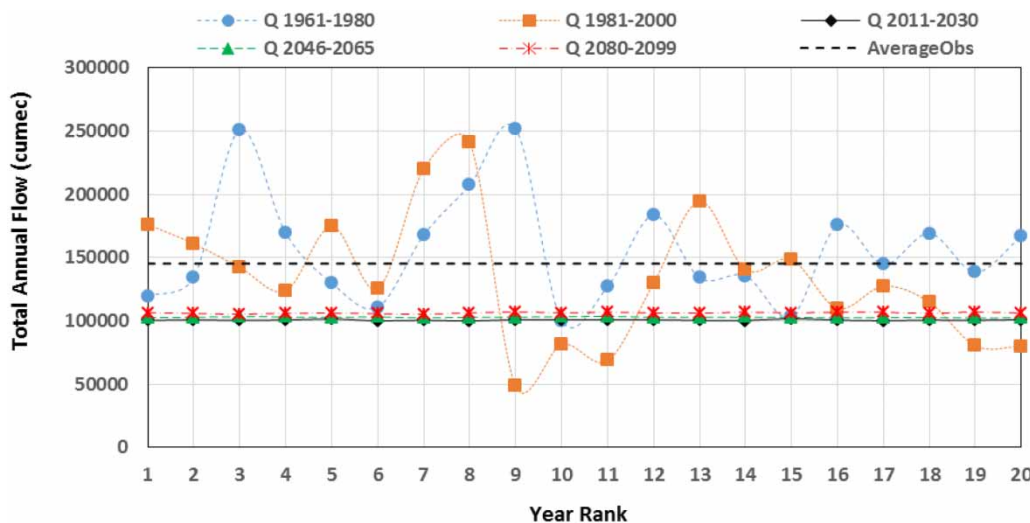
Figure 9 | Comparative plots of annual flow in the baseline and future periods.
