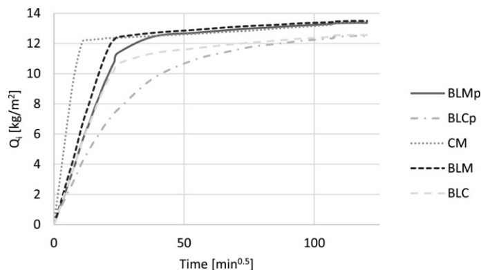
Fig. 7 Capillary rise curves of mortars.
