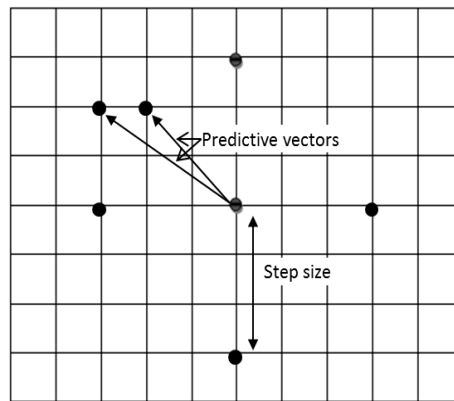
Figure 4. Mean predictive block matching algorithms for the MPBMLY algorithm, including the large search pattern (LSP) and two predictive vectors. Solid circle points (•) correspond to the search points.
