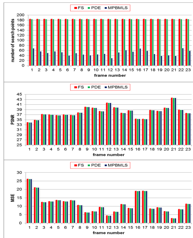
Figure 6. Average number of search points per MB, peak signal-to-noise ratio (PSNR) performance, and mean square error (MSE) of MPBMLS, full search (FS), and partial distortion elimination (PDE) for the “Claire” video sequence of 23 frames.
