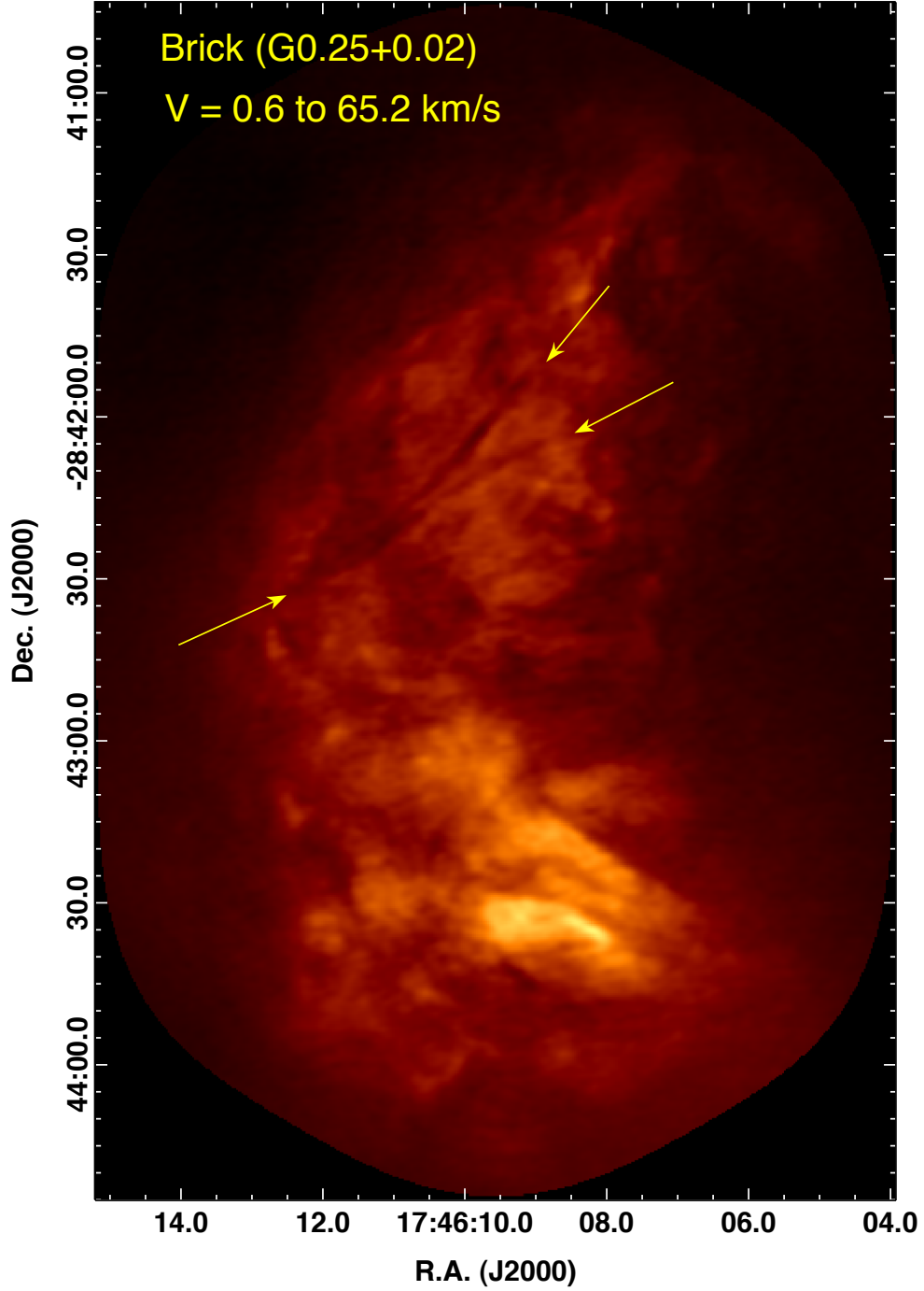
Fig. 1.— A velocity integrated image showing G0.253+0.016 in the \text{HCO}^+ J = 1-0 transition. The velocity range extends from V_{\text{LSR}} = 0.6 \text{ km s}^{-1} to 65.2 \text{ km s}^{-1} . Arrows mark the locations of the two broad line absorption (BLA) filaments. These arrows are retained in Figures 2 through 9.
