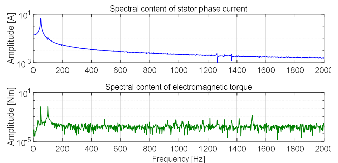
FIGURE 6. Spectral content of stator phase current (top) and developed electromagnetic torque (bottom) in steady-state conditions for machine with R = 54 unskewed rotor bars – results from PWF model
