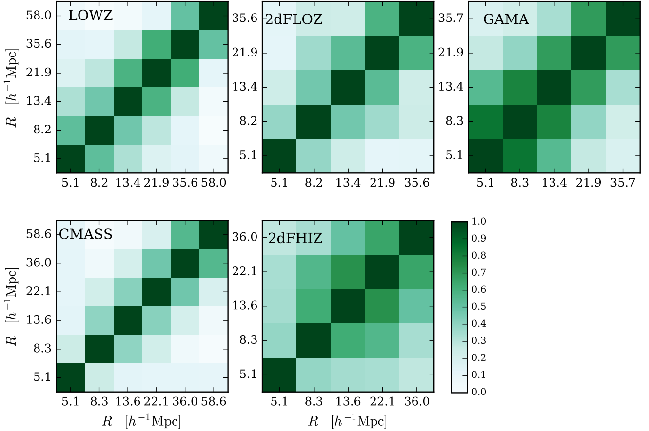
Figure 3. Correlation coefficients, \xi , defined by equation (35), of the covariance matrix of the E_G measurements, determined with each of the five lens samples. These are computed as a combination of the \Upsilon_{\text{gm}} covariance determined from the scatter across the 600 simulation line of sights, the jackknife covariance of \Upsilon_{\text{gg}} and the uncertainty on the RSD parameter, \beta .
