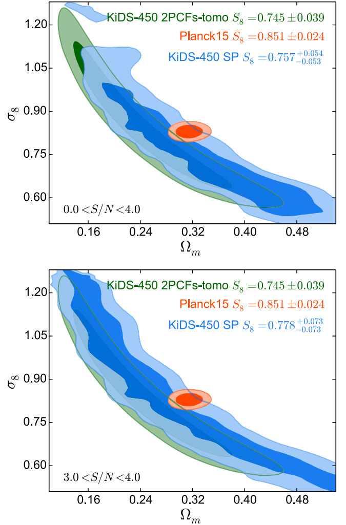
Figure 7. Cosmological constraints on (\Omega_m, \sigma_8) . The 1\sigma and 2\sigma confidence regions are displayed in dark and light areas, respectively. Green contours correspond to KiDS-450 tomographic 2PCFs constraints marginalized over systematics (Hildebrandt et al. 2017), blue to the KiDS-450 shear peak constraints using bins in ranges 0 \leq S/N \leq 4 (top), and 3 \leq S/N \leq 4 (bottom), and red to Planck ‘TT+lowP’ (Planck Collaboration XIII 2016). The top right legend shows the S_8 best value and 68 per cent errors for each study.
