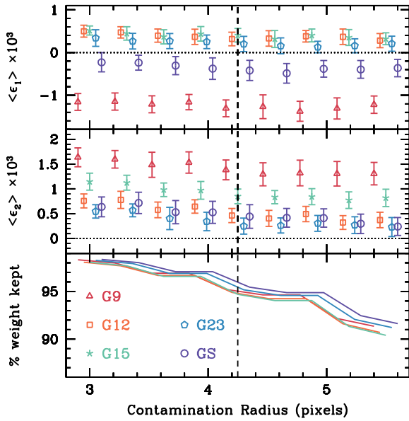
Figure D1. Criterion for masking of neighbours: the additive calibration bias as measured from the weighted average ellipticity \epsilon_1 (upper panel) and \epsilon_2 (middle panel), as a function of the minimum allowed contamination radius. The amplitude of the bias is shown for each of the five KiDS-450 patches (G9, G12, G15, G23, and GS), with points slightly offset along the horizontal axis for clarity. The lower panel shows the decreasing effective number density of objects as the contamination radius cut increases. Our chosen contamination radius cut of >4.25 pixels is shown in dashed.
