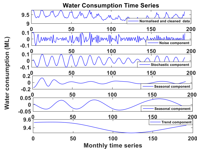
Figure 4. Normalised and cleaned water time series and the first five components obtained by EMD.
