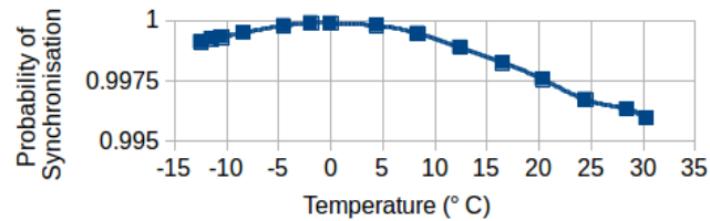
Figure 4: Probability of synchronisation for varying temperatures of a second node.
