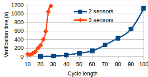
Figure 2: Total time for formal verification of Property 2 for 2- and 3-sensor networks.
