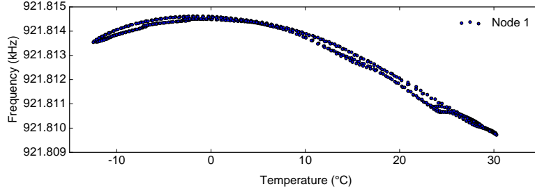
Figure 3: Mica2 hardware clock frequency for different ambient temperatures [LSW09].
