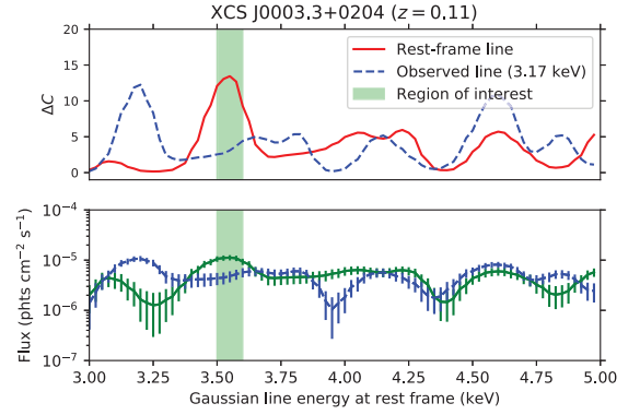
Figure 12. Plot of the change in fit statistic, \Delta C (as in Fig. 4) for the cluster XCS J0003.3+0204. Our standard analysis is given by the red solid line and the blue dashed line shows the change in \Delta C with the analysis performed in the observed frame, i.e. without the blueshifting step (see Section 5.2.1).
