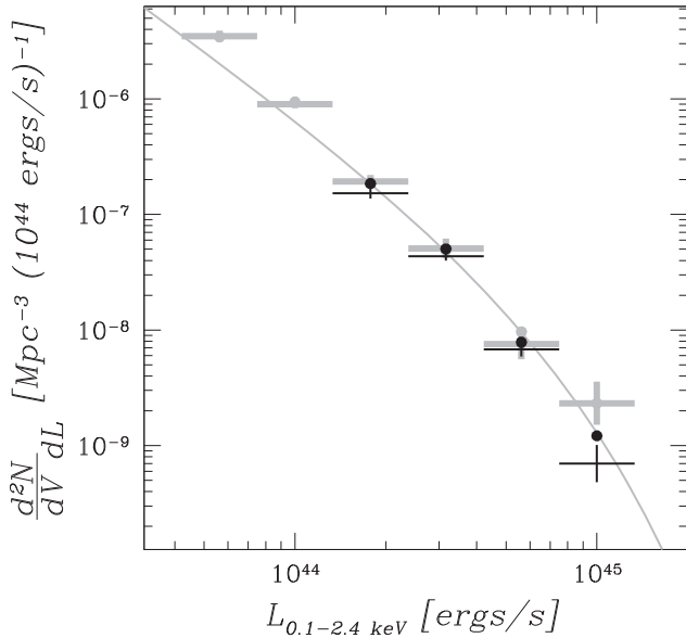
Figure 19. The X-ray luminosity function of the confirmed CODEX galaxy cluster sample in two redshift bins ( 0.1 < z < 0.3 in light grey and 0.3 < z < 0.6 in black). Crosses are data points calculated using spectroscopic redshifts, these redshifts also serve in removing contaminating flux from AGN (see the text); points represent data computed with photometric redshifts only, with no AGN removal. The line shows the Schechter function (Schechter 1976) describing the REFLEX cluster luminosity function (Böhringer et al. 2002).
