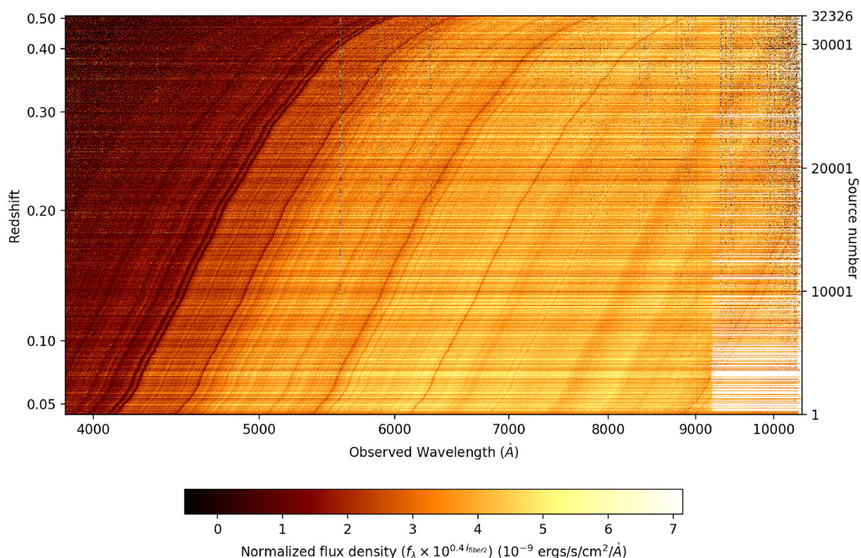
Figure A1. The flux-calibrated spectra corresponding to 32 326 cluster members in the DR16 galaxy cluster catalogue (SCREEN_ISMEMBER.W \geq 0.75). The colour linearly scales with the flux density in each wavelength pixel of a spectrum (units \text{erg s}^{-1} \text{cm}^{-2} \text{\AA}^{-1} ), normalized to the fibre flux of each galaxy. Spectra are sorted according to their redshift (indicated on the y-axis). The observed wavelength scale is logarithmic. The main absorption features visible from z = 0.013 to z = 0.679 are Ca II H + K, G-band, Mg I, NaD, etc. Some galaxies (barely visible here) display emission features, notably [O III] and H \alpha . The white stripes at observed wavelengths beyond 9200 Å represent missing data at wavelengths not covered by the SDSS-I/II spectrograph.
