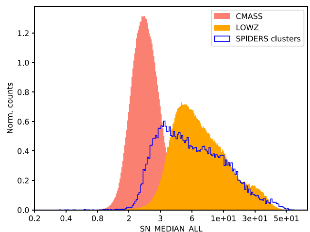
Figure 9. Distribution of the median spectral signal-to-noise ratio ( \text{SN\_MEDIAN\_ALL} ) for all SPIDERS targets. As a comparison, the distributions for the BOSS CMASS and BOSS LOWZ samples are also shown.
