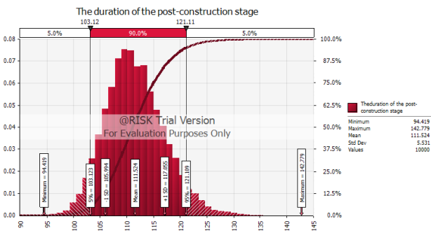
Figure 7. The results of simulating the duration of the post-construction stage of the project.
