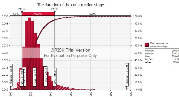
Figure 6. The results of simulating the duration of the construction stage of the project.
