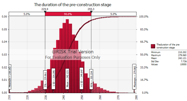
Figure 5. The results of simulating the duration of the pre-construction stage of the project.
