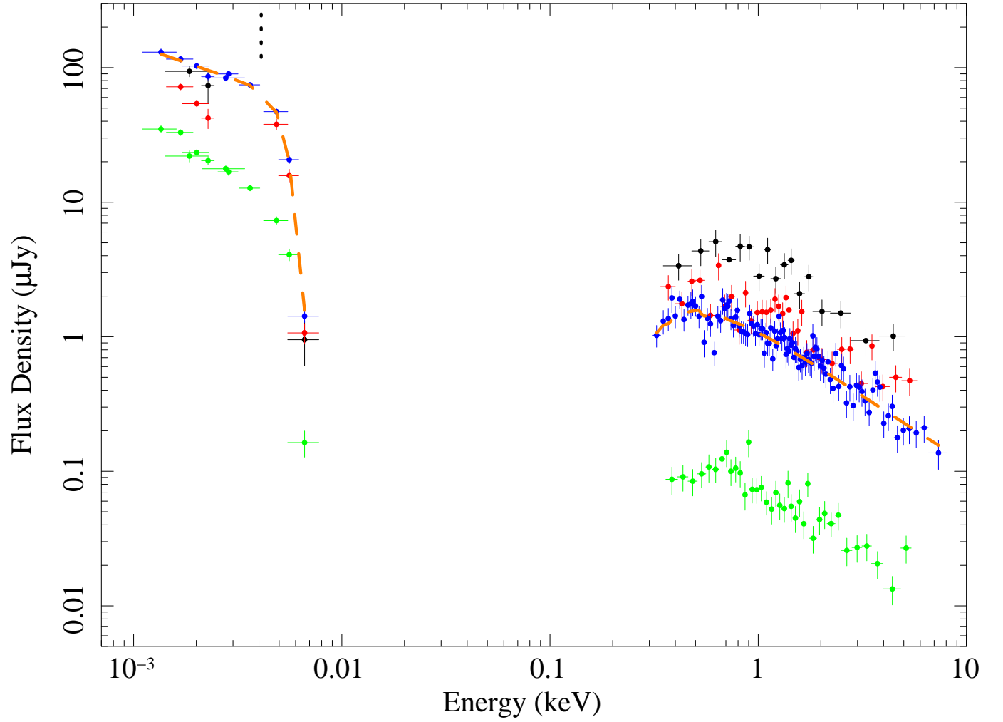
Figure 6. SEDs at 4.5 ks (black), 22 ks (red), 50 ks (blue) and 400 ks (green). The orange long-dashed line connecting the points of the 50 ks SED shows the best-fit model, that is the sum of two broken power laws; the black short-dashed vertical line indicates the position suggested for the synchrotron peak frequency of the first component. The 22 ks and 50 ks SEDs appear flat in the optical, while the 4.5 and especially the 400 ks SEDs show a steeper optical spectrum.
