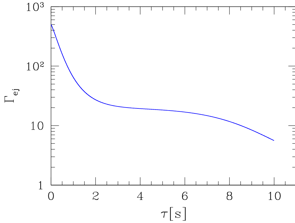
Figure 8. Distribution of Lorentz factor of the ejecta vs time of ejection \tau in seconds. See Sect. 4.6 for more details.
