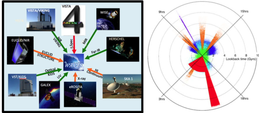
Fig. 5 (left) The facilities ultimately contributing to the WAVES survey. (right) a cylinder-plot showing the region of the Universe probed by WAVES compared to other notable surveys.
