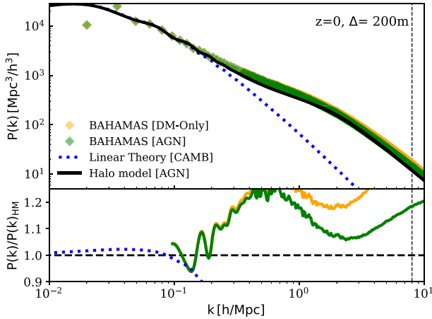
Figure 9. Same as Fig. 7 but for the hydrodynamical ( AGN ) case. The BAHAMAS AGN matter power spectrum is represented by the green symbols. The bottom panel we show the ratios with respect to the baryonic version of the halo model (i.e. using the density profiles and HMF from the BAHAMAS AGN run). The level of agreement between the baryonic halo model and the hydrodynamical simulations is similar to that seen in the comparison of the collisionless halo model and collisionless simulations in Fig. 7.
