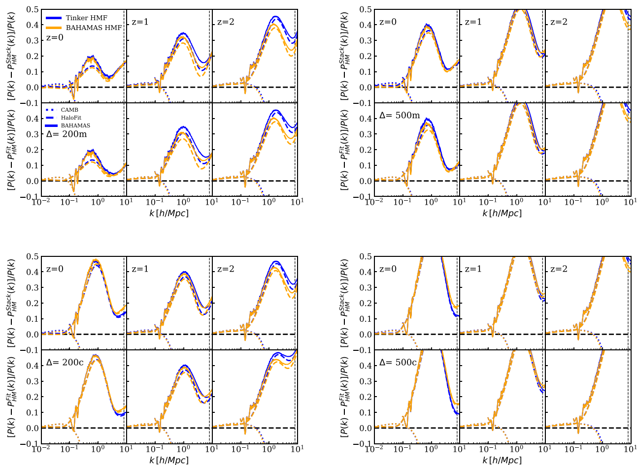
Figure 8. Residual plots between the matter power spectrum and the halo model predictions at three different redshifts for the four different mass definition as follows: top-left \Delta = 200m , top-right \Delta = 500m , bottom-left \Delta = 200c , and bottom-right \Delta = 500c . The top (bottom) row of panels in each plot set correspond to the case where the tabulated profiles directly from the simulations (Einasto fits to) are used in the halo model. The orange (blue) curves correspond to the case where we use the BAHAMAS DM-only simulation (Tinker) HMF. We compare against linear theory predictions using CAMB (dotted curves) and the non-linear HALOFIT prediction (dashed curves) and BAHAMAS DM-only simulation (solid curves). The vertical dotted line represents 0.5 times the Nyquist frequency of the BAHAMAS simulation volume. All models recover the large-scale limit by construction, while the 1-halo/2-halo transition region is (at best, corresponding to the \Delta = 200m case) recovered to 10–15 per cent accuracy. In general, the accuracy decreases with decreasing radial extent of the haloes (due to changing halo mass definition, see text) and increasing redshift.
