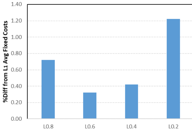
Figure 6: Effect of L value on the fixed cost
