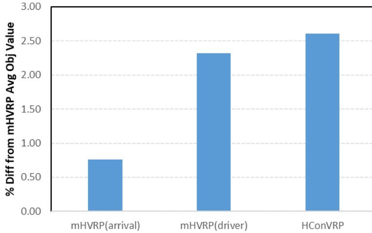
Figure 4: Cost of service consistency - small-scale instances
