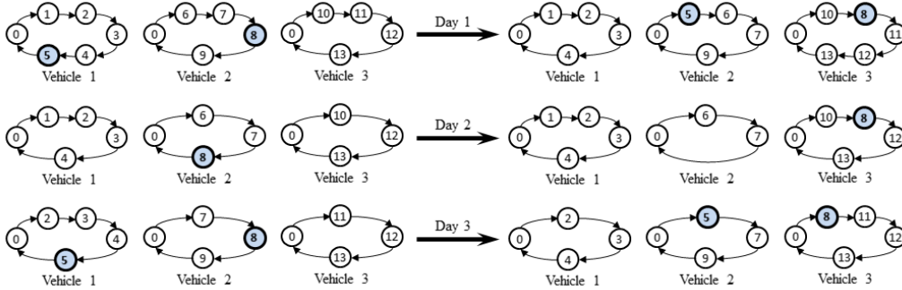
Figure 3: ChangeVehicleChain move
