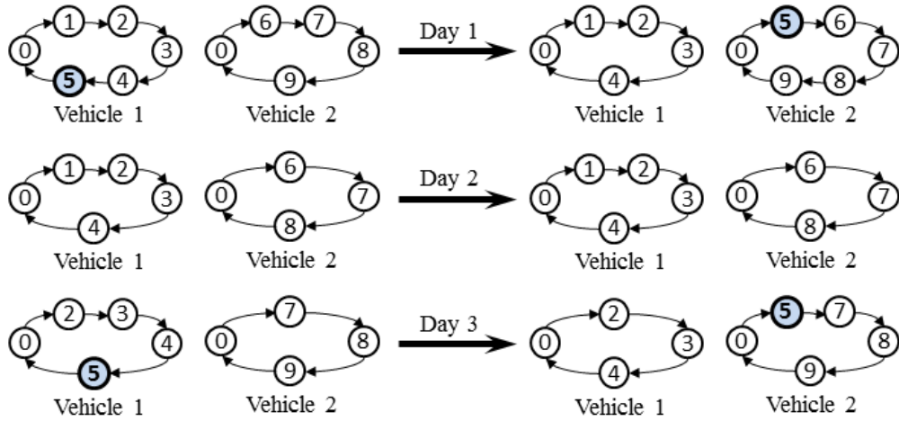
Figure 1: ChangeVehicle move
