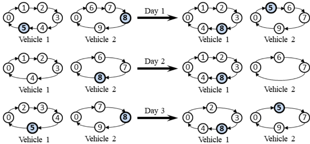
Figure 2: SwapVehicle move
