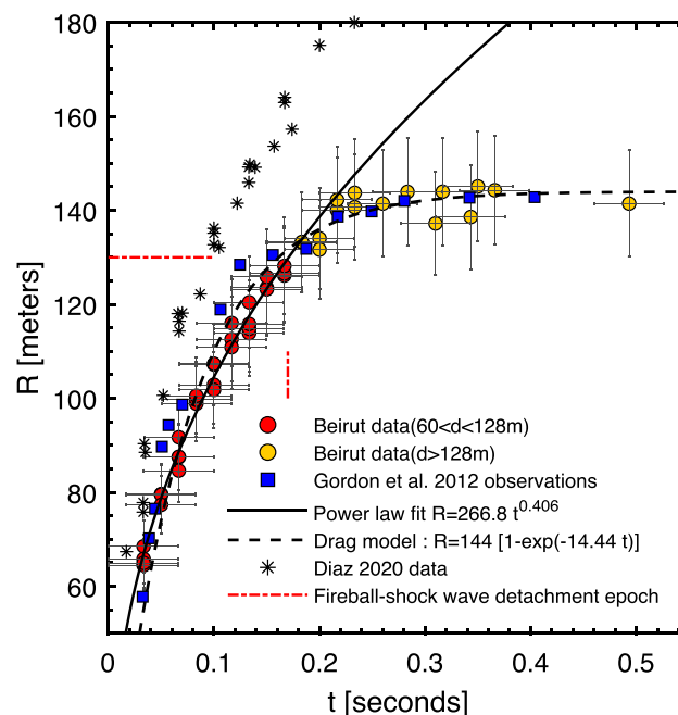
Fig. 7 Fireball radius evolution with time. The red dots are the fireball measurements used in evaluating the TNT equivalence of the explosion, taken at distances less than about 130 m and at times less than about 170 ms. A power law with an exponent of 0.406, which is represented with the black line, fits the data within this time interval and is consistent with the Sedov–Taylor model with spherical geometry and instantaneous energy release. Within the above-mentioned time interval, the fireball measurements are assumed to trace the shock wave evolution. The orange dots are the fireball measurements taken at later time moments, i.e., when the fireball and the shock wave have already detached, until the luminous fireball has reached its final radius. The dashed curve represents a drag theoretical model describing the evolution of the fireball until reaching the stopping distance at about 140 m. The straight dashed red lines represent the time moment and the distance where the shock wave is assumed to detach from the fireball. The blue squares represent the fireball evolution in time from Gordon et al. [7] scaled to the TNT equivalence of the Beirut explosion. Small asterisks show the data from Diaz [5] for comparison
