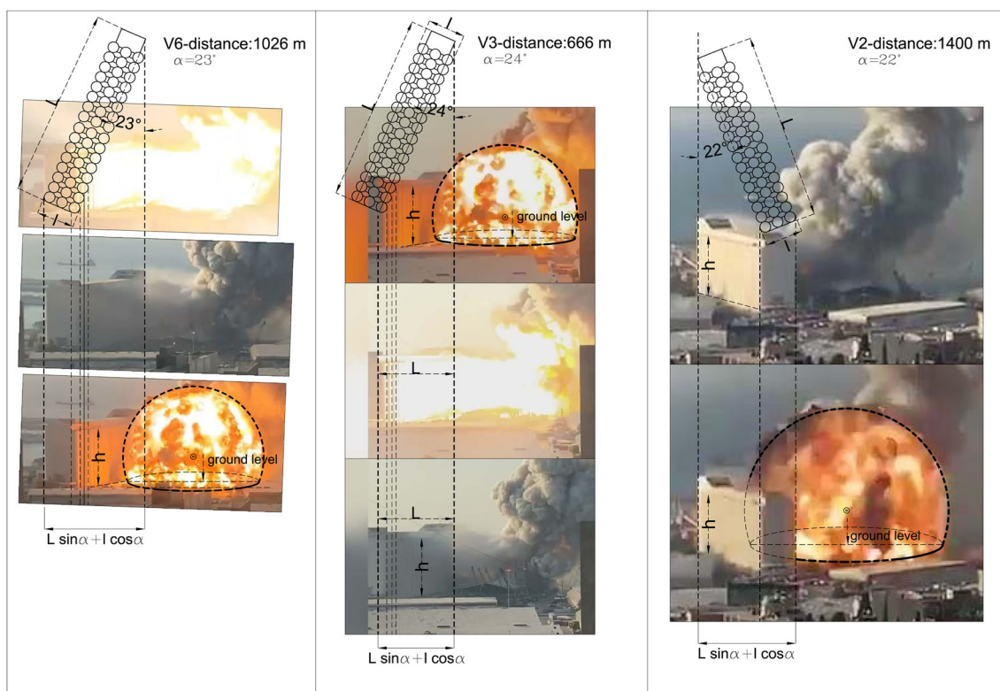
Fig. 4 For each video, the incident angle-of-sight toward the silos long facade is shown along with the actual picture of the silos and the projection lines
