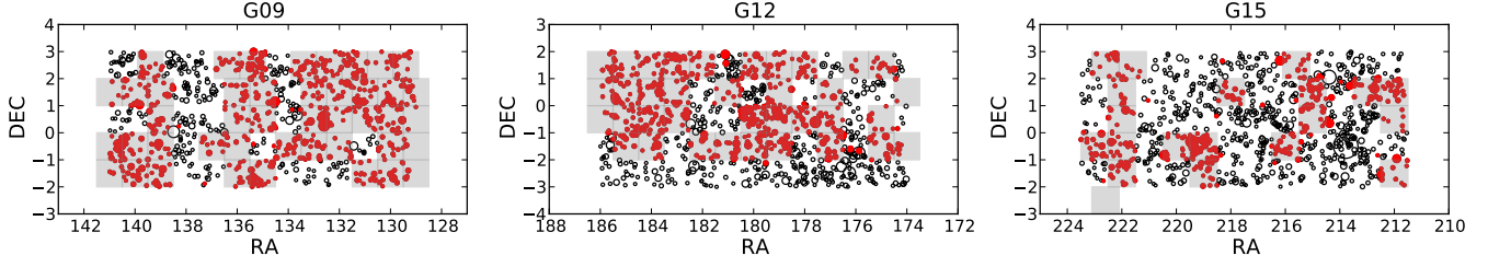
Figure 1. KiDS-ESO-DR1/2 coverage of the three equatorial GAMA fields (G09, G12, G15). Each grey box corresponds to a single KiDS tile of 1 square degree. The black circles represent groups with N_{\text{fof}} \geq 5 in the G^3\text{Cv7} catalogue (R+11). The size of the dots is proportional to the group apparent richness. The filled red circles indicate the groups used in this analysis. These are all groups either inside a KiDS field or whose centre is separated less than 2 h^{-1} \text{Mpc} from the centre of the closest KiDS field.
