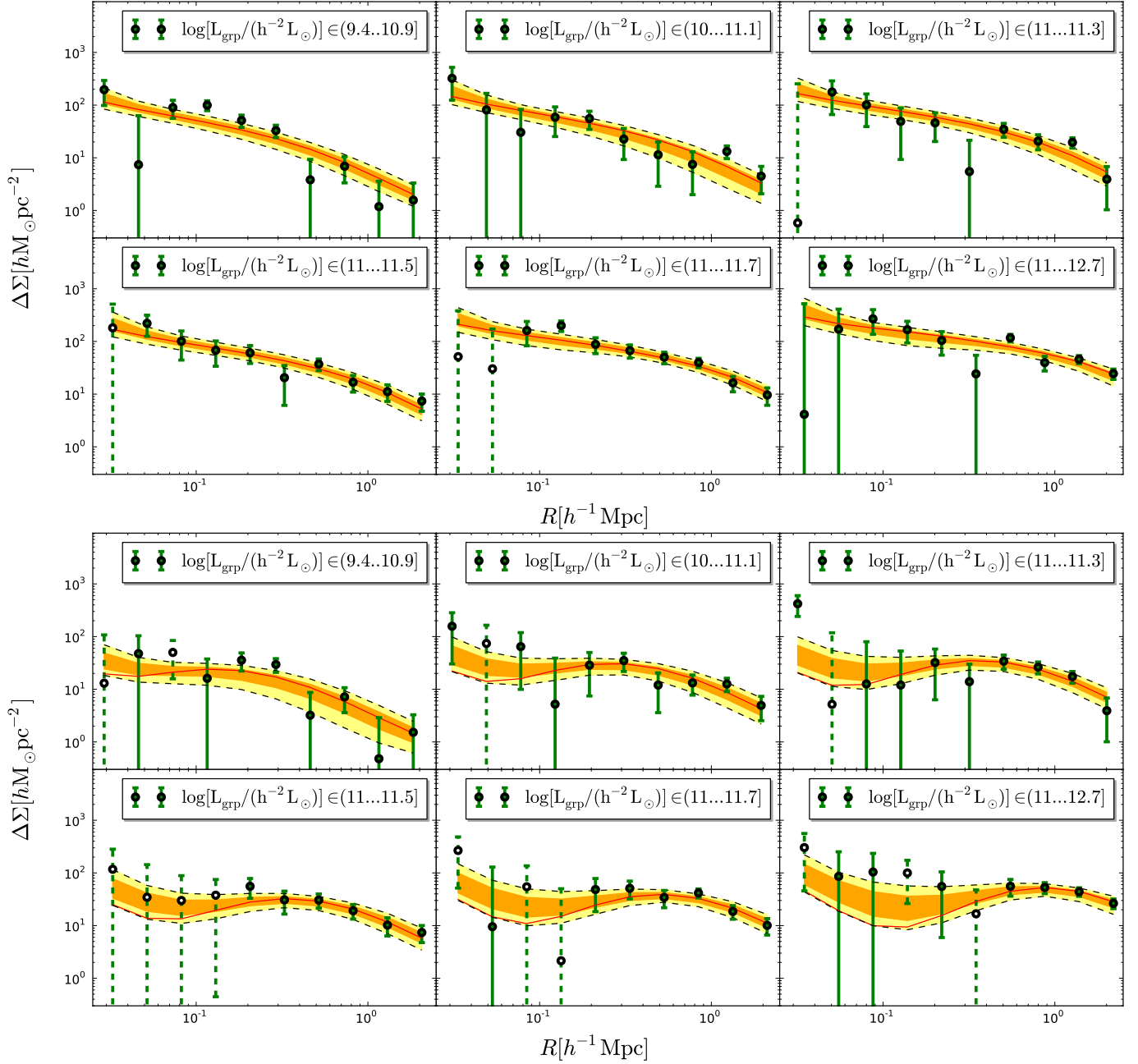
Figure A1. Stacked ESD measured around the groups' IterCen ( upper panel ) and the groups' centre of light Cen ( lower panel ) for 6 group luminosity bins as a function of distance from the group centre. The group luminosity increases from left to right and from top to bottom. The stacking of the signal has been performed considering only groups with N_{\text{fof}} \geq 5 . The error bars on the stacked signal are computed as detailed in section 3.4. The orange and yellow bands represent the 68 and 95 percentile of the model around the median and the red lines indicate the best fit model.
