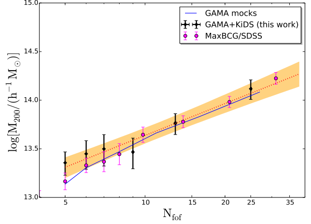
Figure 16. Group halo mass as a function of the richness ( N_{\text{fof}} ). We use here only groups with at least 5 members brighter than r_{AB} = 19.8 . The richness of the groups is not corrected to account for the fainter galaxies not targeted by GAMA. The red line shows the best fit power-law relation to the data points. Our estimate of the 1-sigma dispersion around this relation is shown as the orange area. The blue line shows the mass-richness relation derived from the GAMA mocks using the same selection function applied to the data. The magenta points show the result of a weak lensing analysis of 130,000 groups and clusters of galaxies in the Sloan Digital Sky Survey (Johnston et al. 2007).
