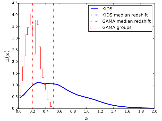
Figure 2. Redshift distribution of the GAMA groups used in this analysis (red histogram) and the KiDS galaxies (blue lines). In the case of the GAMA groups, we use the spectroscopic redshift of the groups with at least 5 members (R+11), while for the KiDS galaxies the redshift distribution is computed as a weighted sum of the posterior photometric redshift distribution as provided by BPZ (Benítez 2000). The weight comes from lensfit , used to measure the shape of the objects (Miller et al. 2007). The two vertical lines show the median of the redshift distribution of the GAMA groups and of the KiDS sources. The two peaks in the redshift distribution of the GAMA groups are physical (and not caused by incompleteness), due to the clustering of galaxies in the GAMA equatorial fields.
