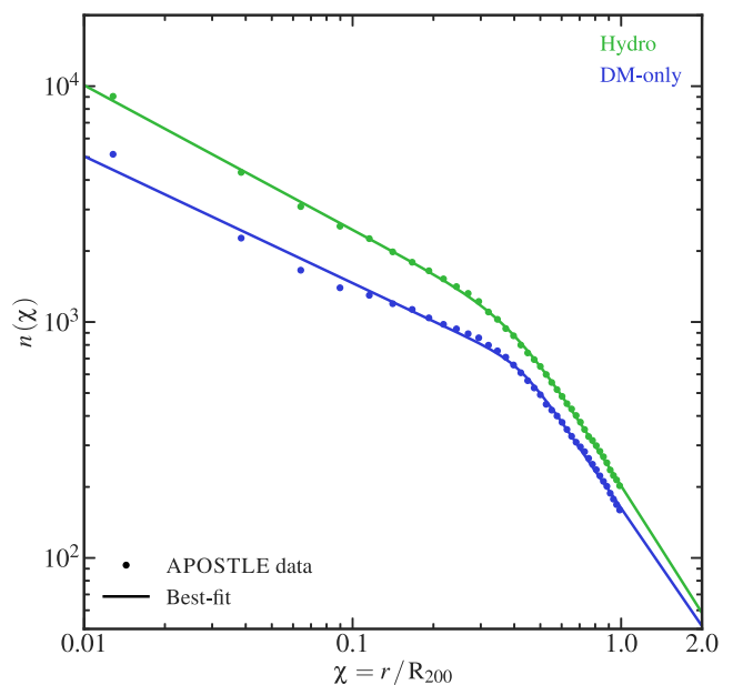
Figure C1. Fits to subhalo number density profiles in DM-only and hydrodynamic simulations. The points show averaged radial profiles for four APOSTLE haloes. To obtain better statistics, these points were also averaged over 5 Gyr of cosmic time; see Sawala et al. (2017) for details. The solid lines show the best-fitting double power laws (see the main text for the best-fitting parameters).
