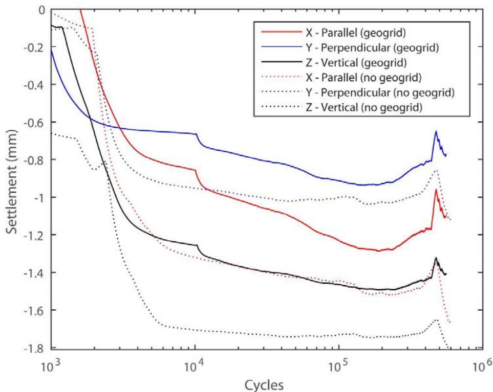
Figure 8 Settlement curves for sub-ballast/subgrade settlement
