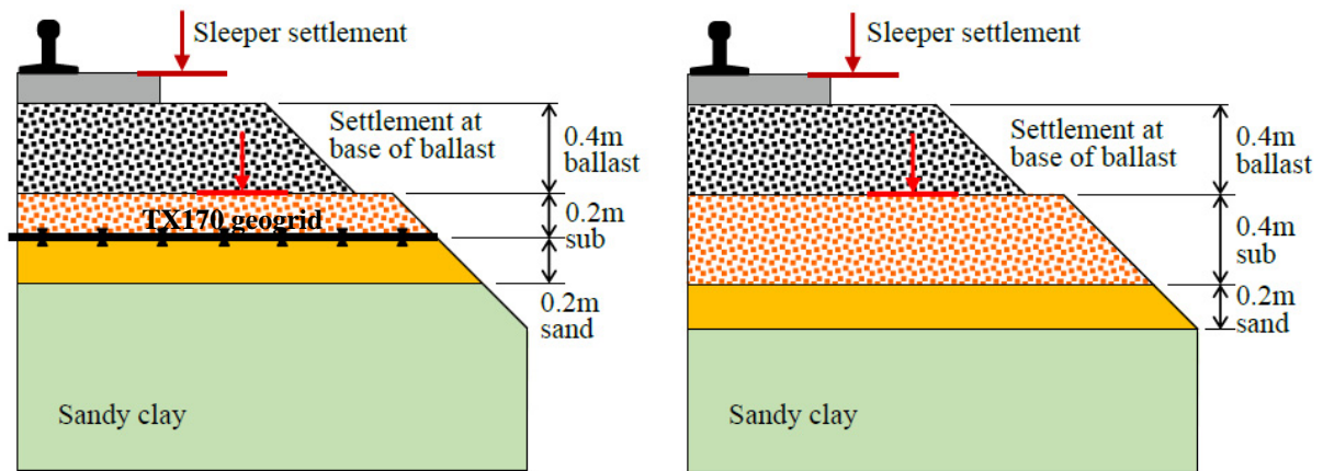
Figure 2. Test setup for stabilised sub-ballast testing at PNF St Petersburg, stabilised with TX170 (left) and control (right). Note that the Ev2 value on the surface of the stabilised sub-ballast is increased by 56% despite the reduced sub-ballast thickness
