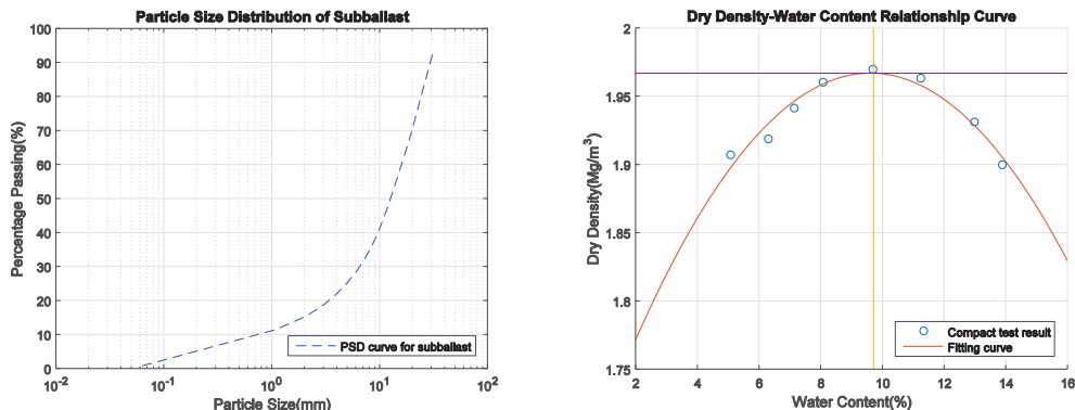
Figure 6 Grading curve for sub-ballast aggregate use in GeoTT testing (left) and dry density/moisture content curve for manufactured clay subgrade (right).
