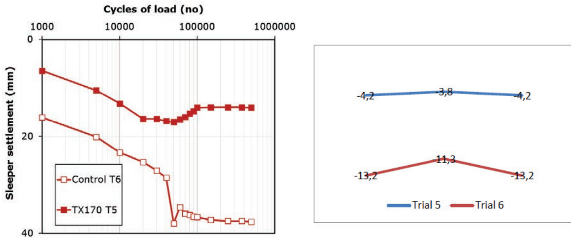
Figure 4. Sleeper settlement curves for PNF St Petersburg testing (left) showing improved retention of track level with TriAx- stabilised sub-ballast and settlement within the sub-ballast layer (right) for the same tests. Note that the settlement of the sub-ballast may include some settlement in formation level
