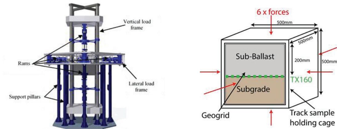
Figure 5. GeoTT test rig schematic (left) and test setup for stabilised sub-ballast over soft subgrade test.
