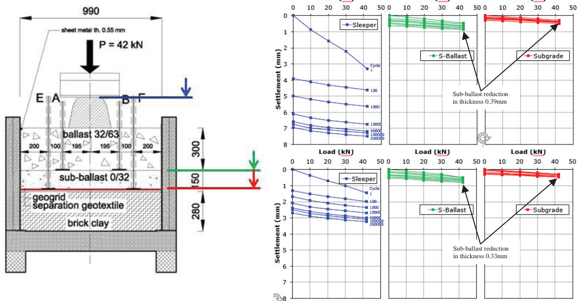
Figure 1 – Test setup at Czech Technical University, Prague (left) and settlement results (right) for SS30 biaxial geogrid (top) and TX160 hexagonal geogrid (bottom) showing marked difference in settlement of ballast over 250,000 cycles of a 42kN load.
