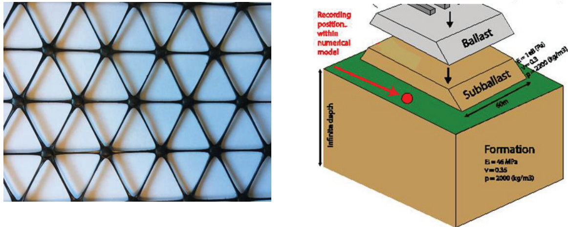
Figure 7. TriAx TX160 geogrid used in GeoTT simulation (left) and recording position for horizontal forces and soil numerical properties (right).
