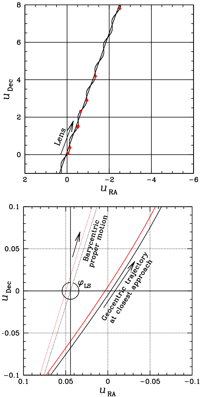
Figure 15. Top panel: path of the lens with respect to the source, the position of the source being fixed at (0, 0) . The direction of motion is shown by an arrow. The black straight line is the lens path without parallax, and the wavy line is the path including parallax. Red points mark the epochs of HST observations. u_{RA} and u_{Dec} are the R.A. and decl. components of the lens–source separation, in units of \theta_E . Bottom panel: enlarged view of the lens trajectory with respect to the source around closest angular approach. Black lines correspond to the u_{0,-} solution, which is the preferred solution, and the red lines show the less preferred u_{0,+} solution. In both cases, the barycentric trajectories (no parallax), shown by dotted lines, pass on the north side of the source. The geocentric trajectory (i.e., the trajectory as seen by an observer on Earth, which includes parallax) of the u_{0,+} solution (shown by the solid red line) passes on the north side of the source, but the trajectory of the u_{0,-} solution (shown by the black solid line) passes to the south. The u_{0,-} solution is used in our analysis presented here. It is worth noting, however, that the derived \theta_E , and hence the mass of the lens, is nearly identical for both solutions. \varphi_{LS} is the PA of the barycentric proper motion of the lens with respect to the source (i.e., no parallax), as shown here.
