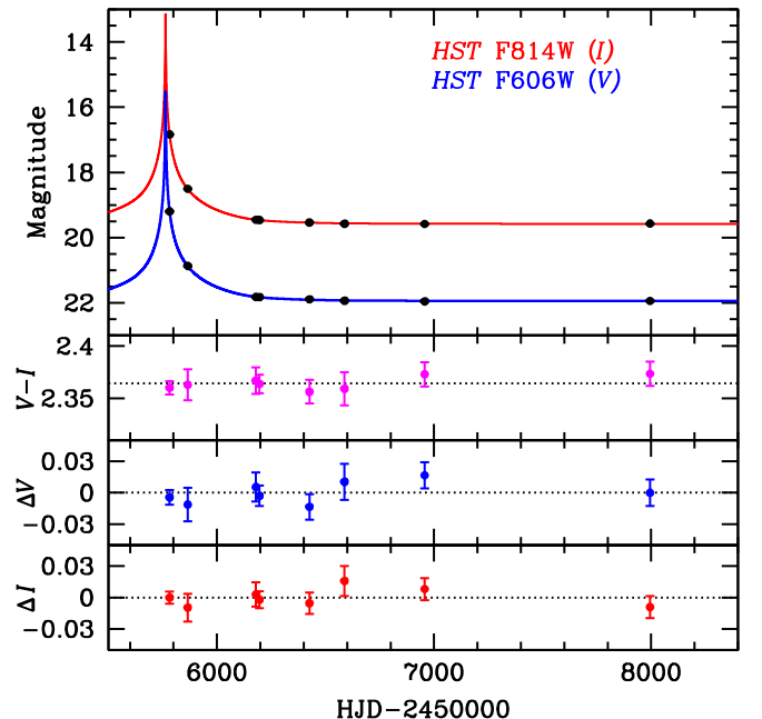
Figure 13. Top panel: photometry of MOA-11-191/OGLE-11-462, obtained with HST over 6 yr at eight epochs in the F606W ( V ) and F814W ( I ) filters (black filled circles), along with our final model fits from Section 8.2 (red and blue curves). Errors on the photometry are smaller than the plotting points. The second panel plots the observed values of V - I , showing that the source color remained constant to within \sim 0.01 mag during the entire 6 yr duration. The third and fourth panels show that the residuals, V_{\text{obs}} - V_{\text{model}} and I_{\text{obs}} - I_{\text{model}} , at the epochs of the HST observations are consistent with zero within the measurement uncertainties (see Section 8.2 for more details and discussion). (The data used to create this figure are available.)
