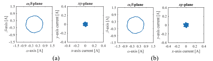
Fig. 17: Effect of stator resistance mismatch (as compared to R_{s1} used in Figs. 13-14) on sub-space currents. (a) 50% R_{s1} ; (b) 200% R_{s1} .
