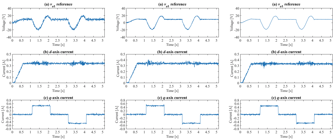
Fig. 7: Measurement noise effect and its compensation. (Left col.) R = 0.0001 \cdot I ; (Middle col.) R = 0.001 \cdot I ; (Right col.) R = 0.01 \cdot I .
