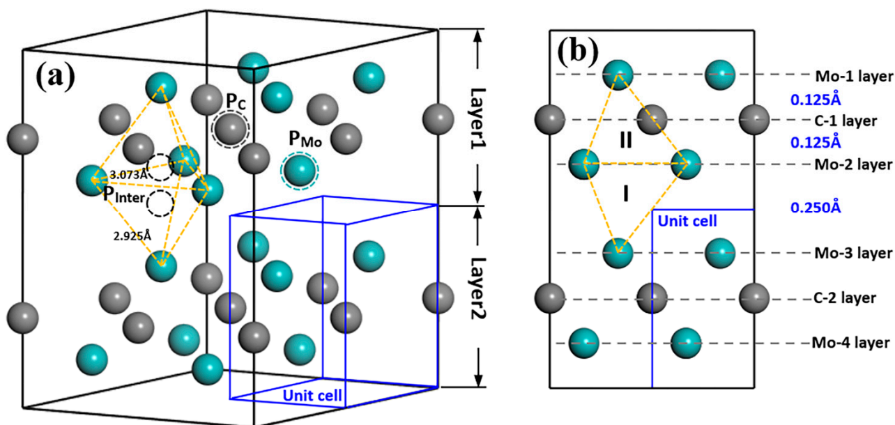
Figure 1. Schematic diagram of Mo_2C structure of 2 \times 2 \times 2 supercell (a) and along [2\bar{1}10] direction (b). Cyan and grey balls represent Mo and C atoms; cyan and grey dashed circles are the positions that are used to form vacancy and substitution defects; yellow dashed frames are the tetrahedrons that Mo atoms formed inside the layer (type II) and between two layers (type I) and the black dashed circles are the tetrahedral position inside the tetrahedrons; blue frame refers to the Mo_2C unit cell. P_{Mo} and P_C represent the positions of the Mo and C atoms, while P_{Inter} refers to the position for interstitial atoms in the structure.
