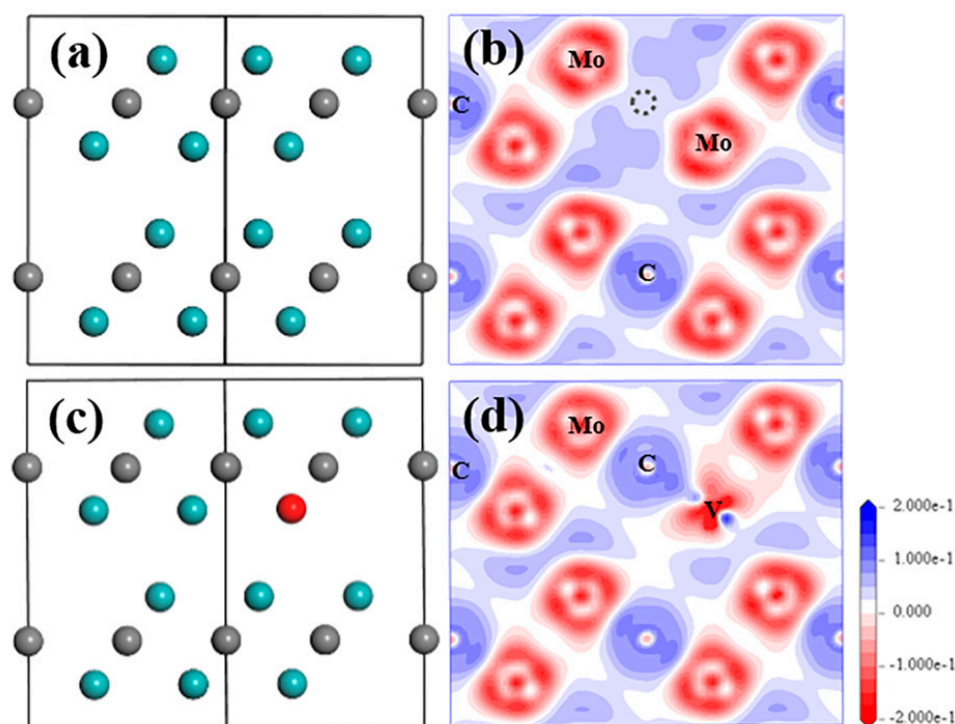
Figure 2. Structure model and electron density difference distribution (EDDD) after optimization in the (11\bar{2}0) plane of \text{Mo}_2\text{C} supercell with V-related defect of (a,b) \text{V}_\text{C} and (c,d) \text{S}_{\text{V-Mo}} . Cyan and grey balls represent Mo and C atom, red ball represent V atom; grey dashed circle shows the \text{V}_\text{C} position.
