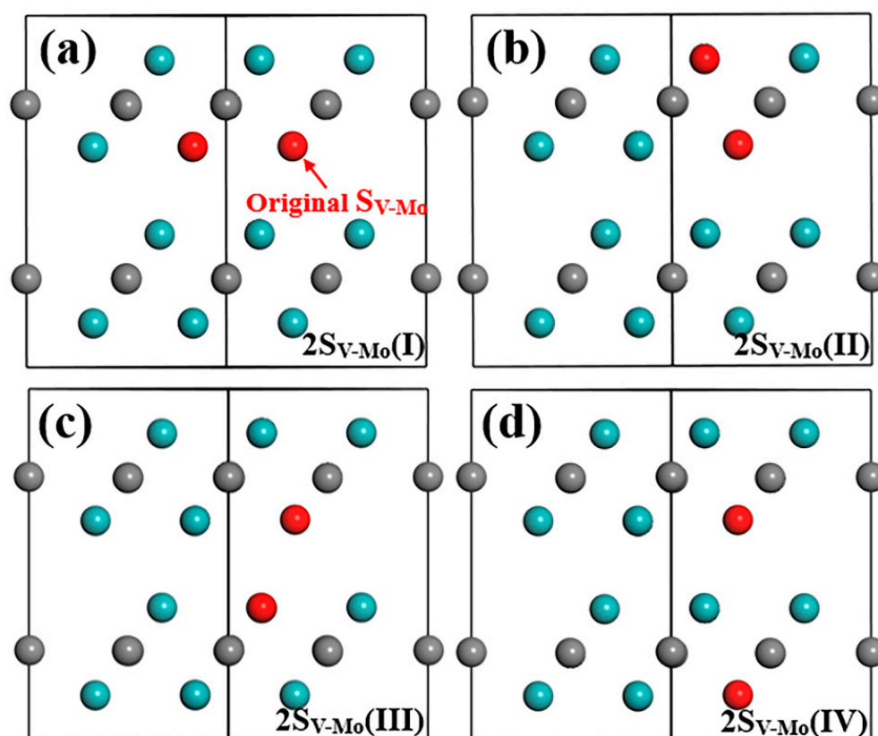
Figure 7. Structure model after optimization in (\bar{1}\bar{1}20) plane of \text{Mo}_2\text{C} supercell with two \text{S}_{\text{V-Mo}} defects: (a) original \text{S}_{\text{V-Mo}} + \text{S}_{\text{V-Mo}} in Mo-2 layer (same layer), (b) original \text{S}_{\text{V-Mo}} + \text{S}_{\text{V-Mo}} in Mo-1 layer (different layer in Layer1), (c) original \text{S}_{\text{V-Mo}} + \text{S}_{\text{V-Mo}} in Mo-3 layer (different layer in Layer2) and (d) original \text{S}_{\text{V-Mo}} + \text{S}_{\text{V-Mo}} in Mo-4 layer (different layer in Layer2). Cyan and grey balls represent Mo and C atom, red ball represents V atom.
