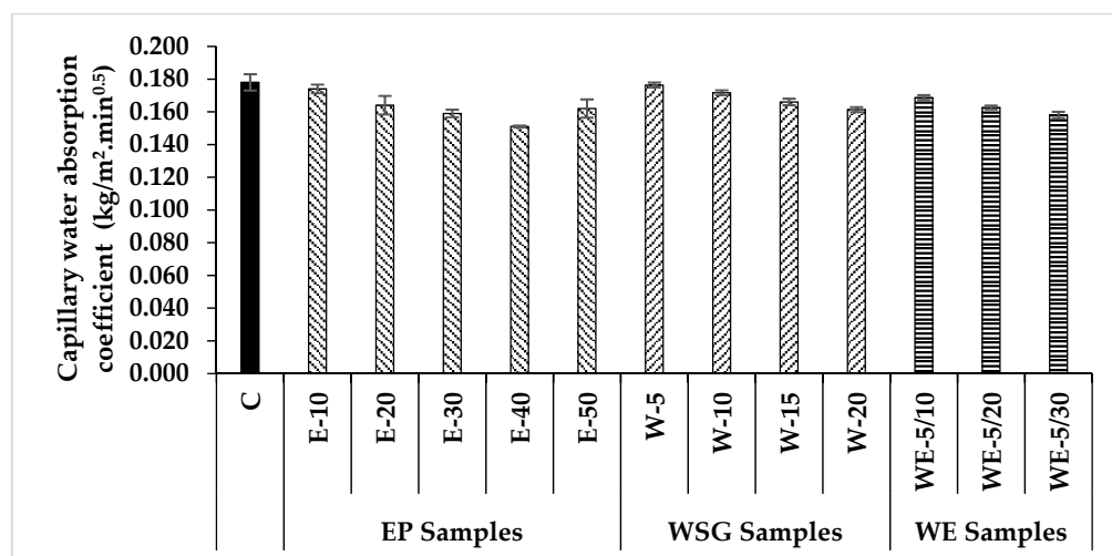
Figure 9. Capillary water absorption results.
