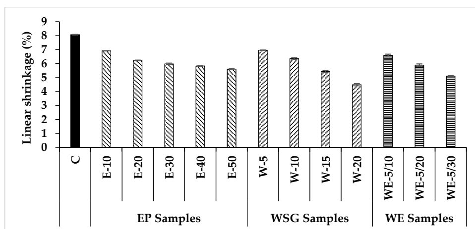
Figure 10. Linear shrinkage results.
