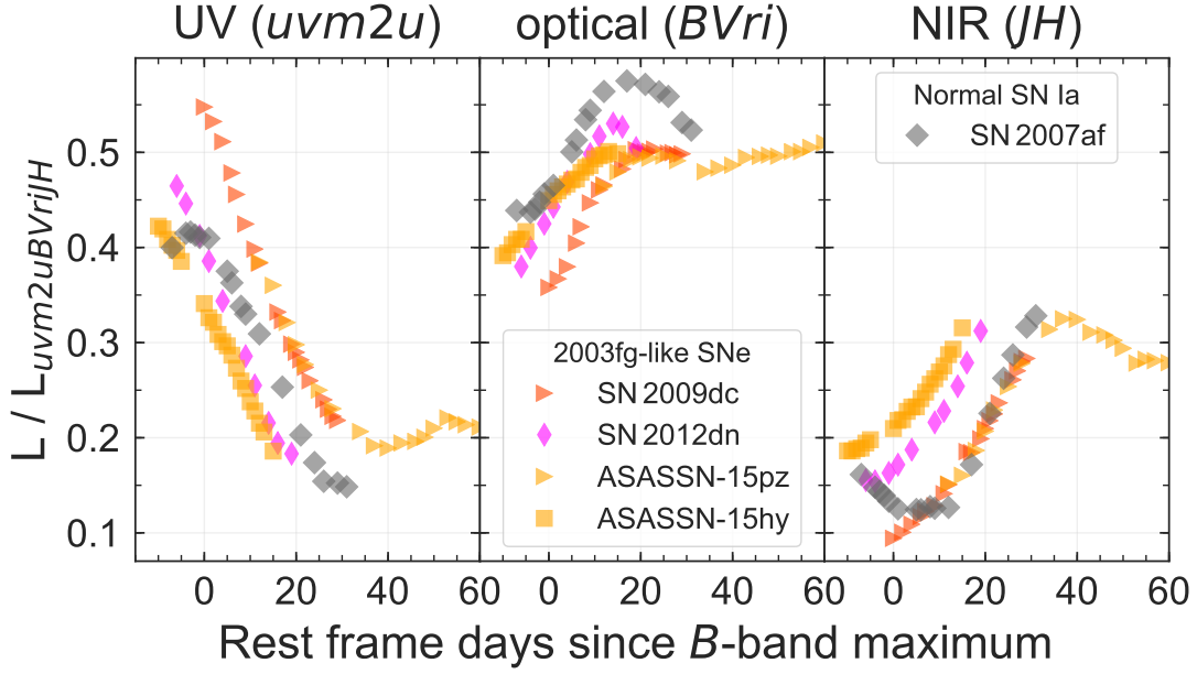
Figure 12. Fractions of pseudo-bolometric luminosity of 2003fg-like SNe in UV ( \sim \lambda 2200 - 4200 ), optical ( \sim \lambda 4200 - 7300 ) and NIR ( \sim \lambda 7300 - 16,000 ) regions. Unlike normal SNe Ia that have the optical region accounting for \sim 80\% of the luminosity, 2003fg-like SNe all show a significant fraction of luminosity in the UV and NIR. The time evolution of the fractions also shows the flux redistribution from UV to NIR.
