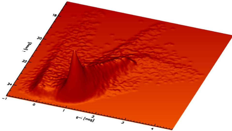
Figure 19. 3D histogram of the i , g-i CMD. The view is from the faint to the brighter limit of the CMD. Note that in this CMD we are plotting all the stars with at least one measurement in g and i bands. The Z-axis is in arbitrary units. From bluer to redder colors the relatively shallow sequences are associated with YMS, RSG, and AGB stars. The steady increase in the star counts present in the central regions is associated with RG stars. The main peak is associated with RC stars.
