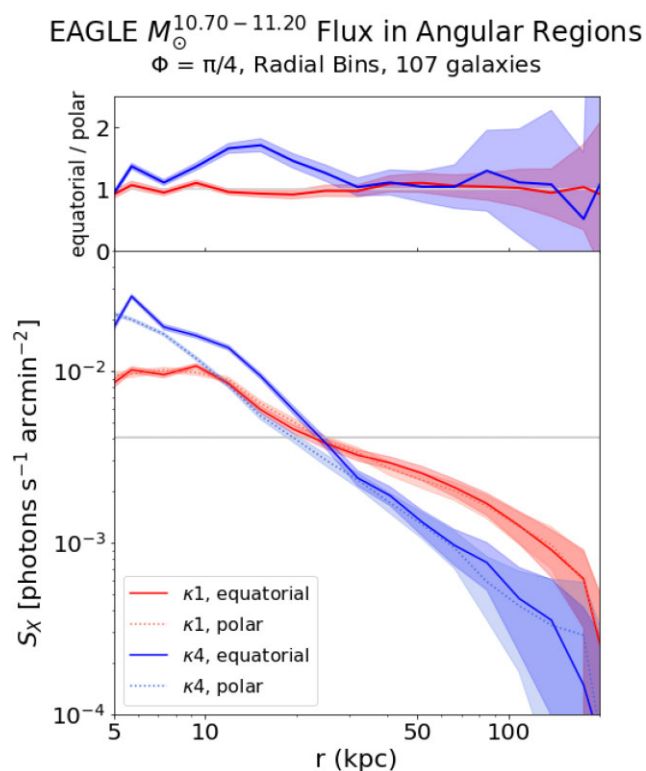
Figure 6. Flux across the 0.2–1.5 keV band divided into equatorial and polar axis regions using \Phi = \pi/4 regions. Disc galaxies ( \kappa 4 ) show greater flux along equatorial than polar regions from 10 to 30 kpc. Spheroidal galaxies ( \kappa 1 ) unsurprisingly do not show any azimuthal dependence, even though they are rotated according to their stellar kinematics. The top panel shows the ratio of the equatorial to polar emission.
