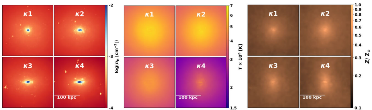
Figure 9. Physical property stacked maps of the hot gas within 200 \times 200 kpc panels: hydrogen number density (left-hand panels), temperature (middle panels), and metallicity (right-hand panels). Each panel set shows the four subsamples: \kappa 1 (top left), \kappa 2 (top right), \kappa 3 (bottom left), and \kappa 4 (bottom right). Higher \kappa galaxies have more elliptical extended gas CGMs beyond the disc, which are slightly lower density than spheroids. The temperature panels show cooler gas around discs than spheroids, indicative of discs living in lower mass haloes. Bipolar metal-enriched outflows are apparent in disc galaxies.
